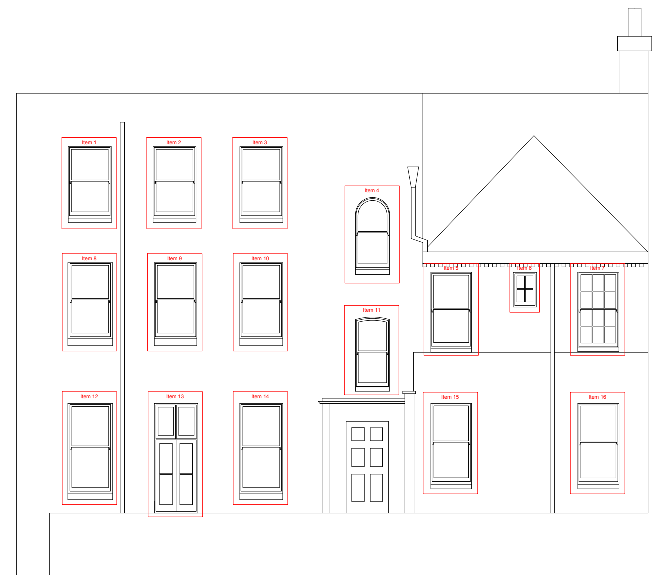
Rear (North) Elevation
