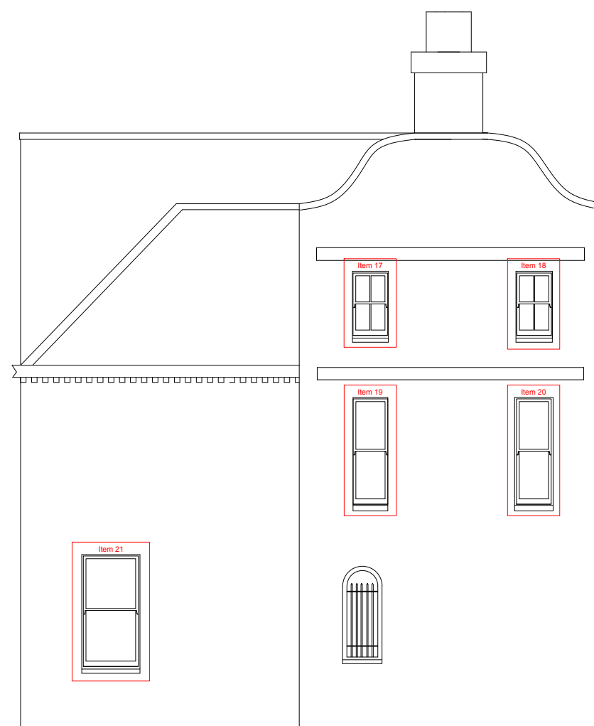
LHS (South) Elevation
