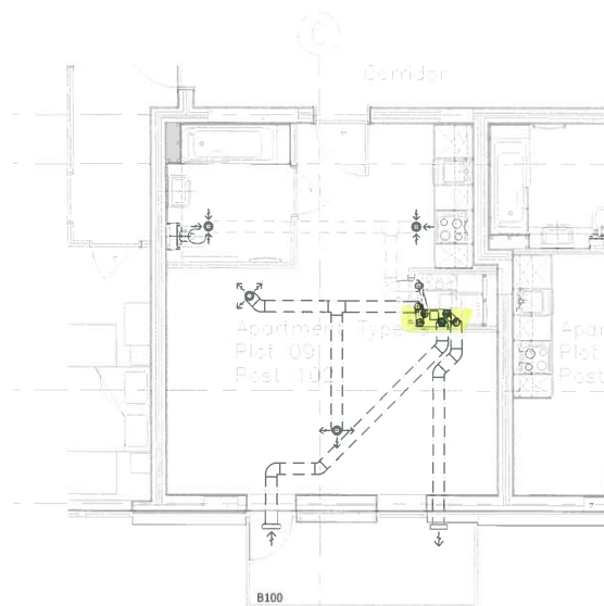
VENTILATION SERVICE
