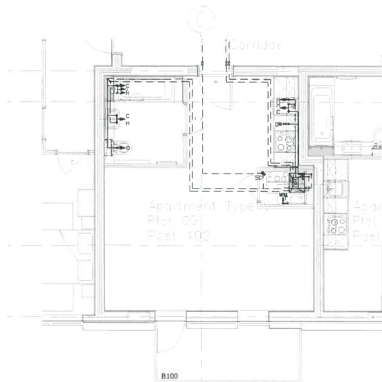
WATER SERVICE
