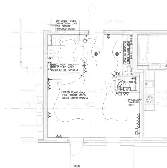
ELECTRICAL SERVICE
