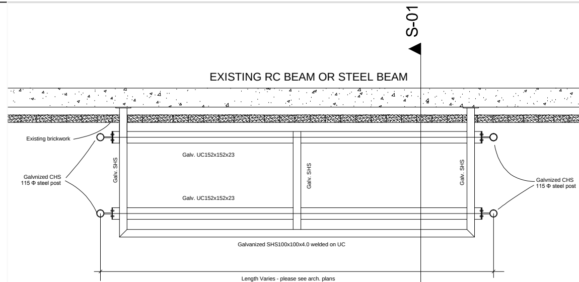
Steel structure Plan 1:50
