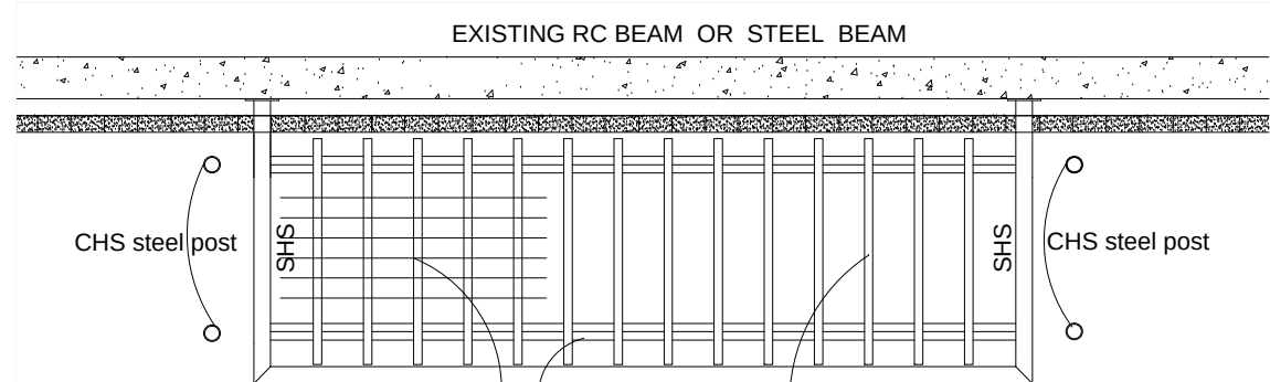
Steel structure Plan 1:50
