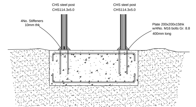
Footing Detail Section-1:50
