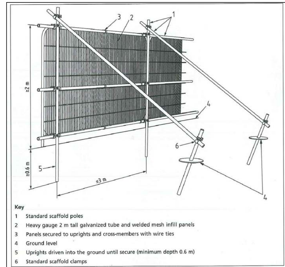
Tree Protection Barrier Specification
