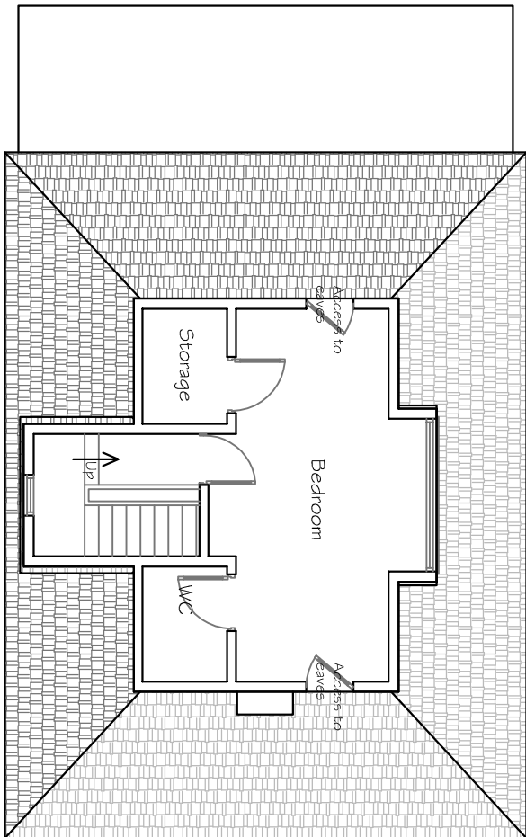
EXISTING FIRST FLOOR PLAN 1 : 100 A3
