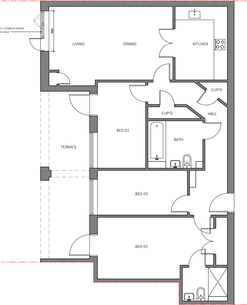
PROPOSED FLOOR PLAN 1:100
