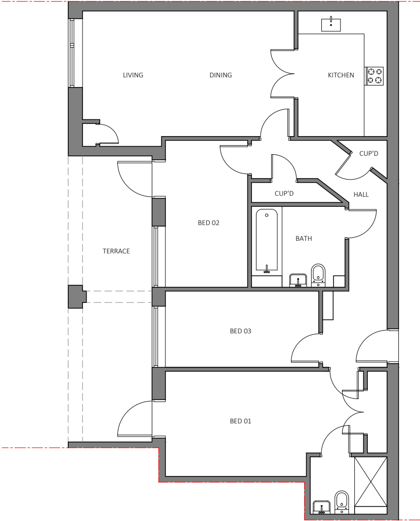
EXISTING FLOOR PLAN 1:100
