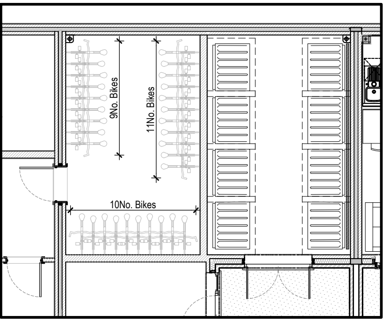
Block A Bike Store - 30 Bikes Block A Bin Store - 1100 Litre Eurobins, 8 number Scale - 1:100
