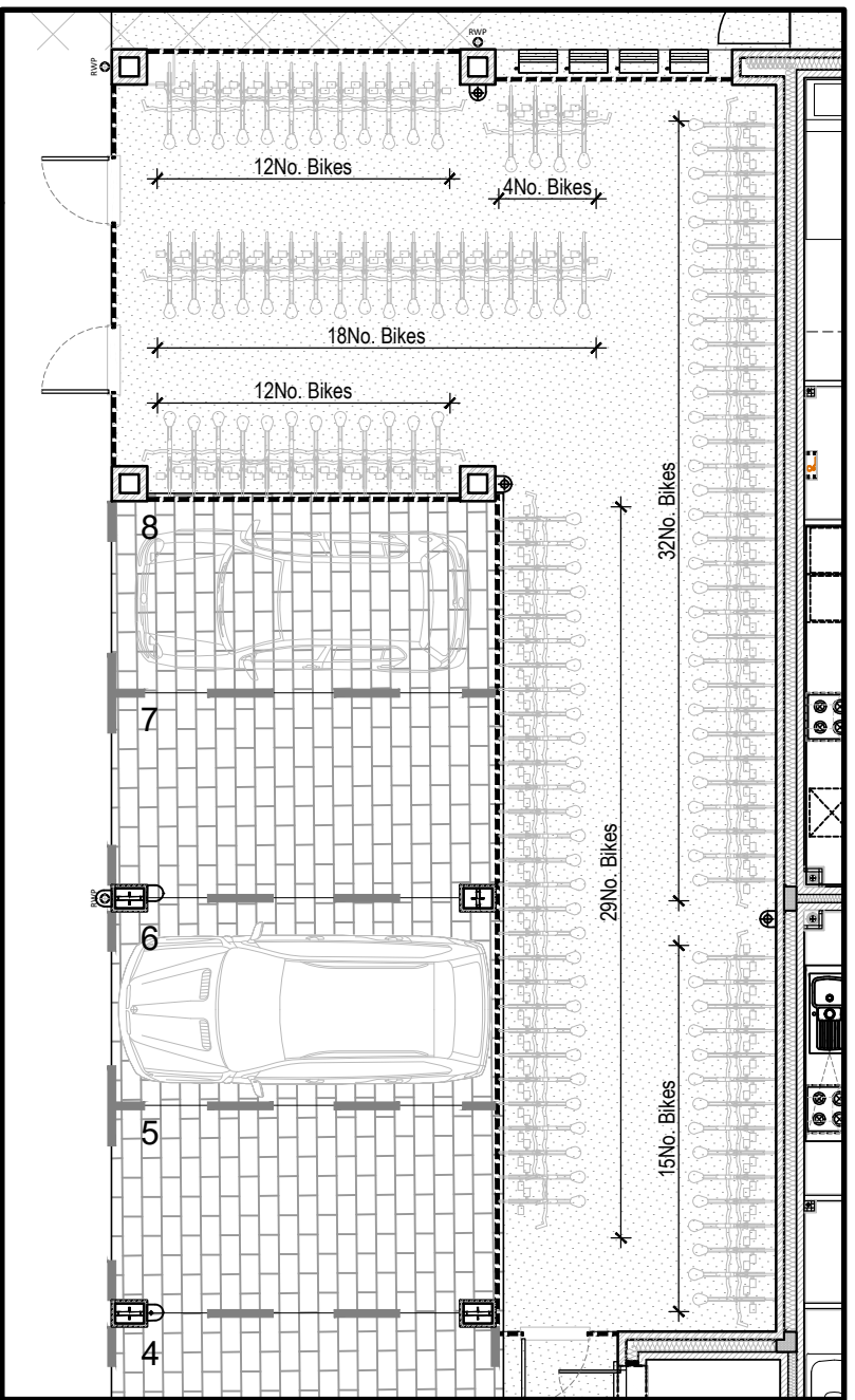
Block B Bike Store - 122 Bikes Scale - 1:100
