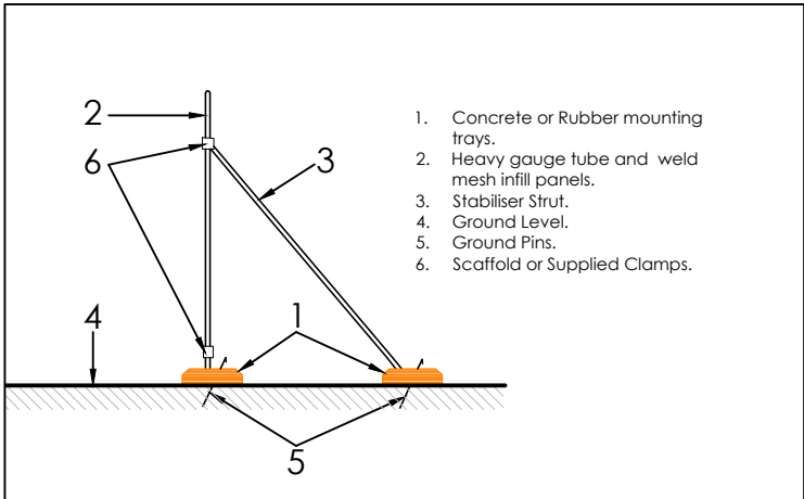
Tree protection Detail (Section)
