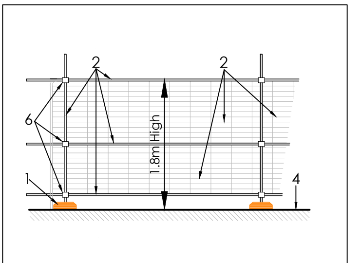
Tree protection Detail (Elevation)
