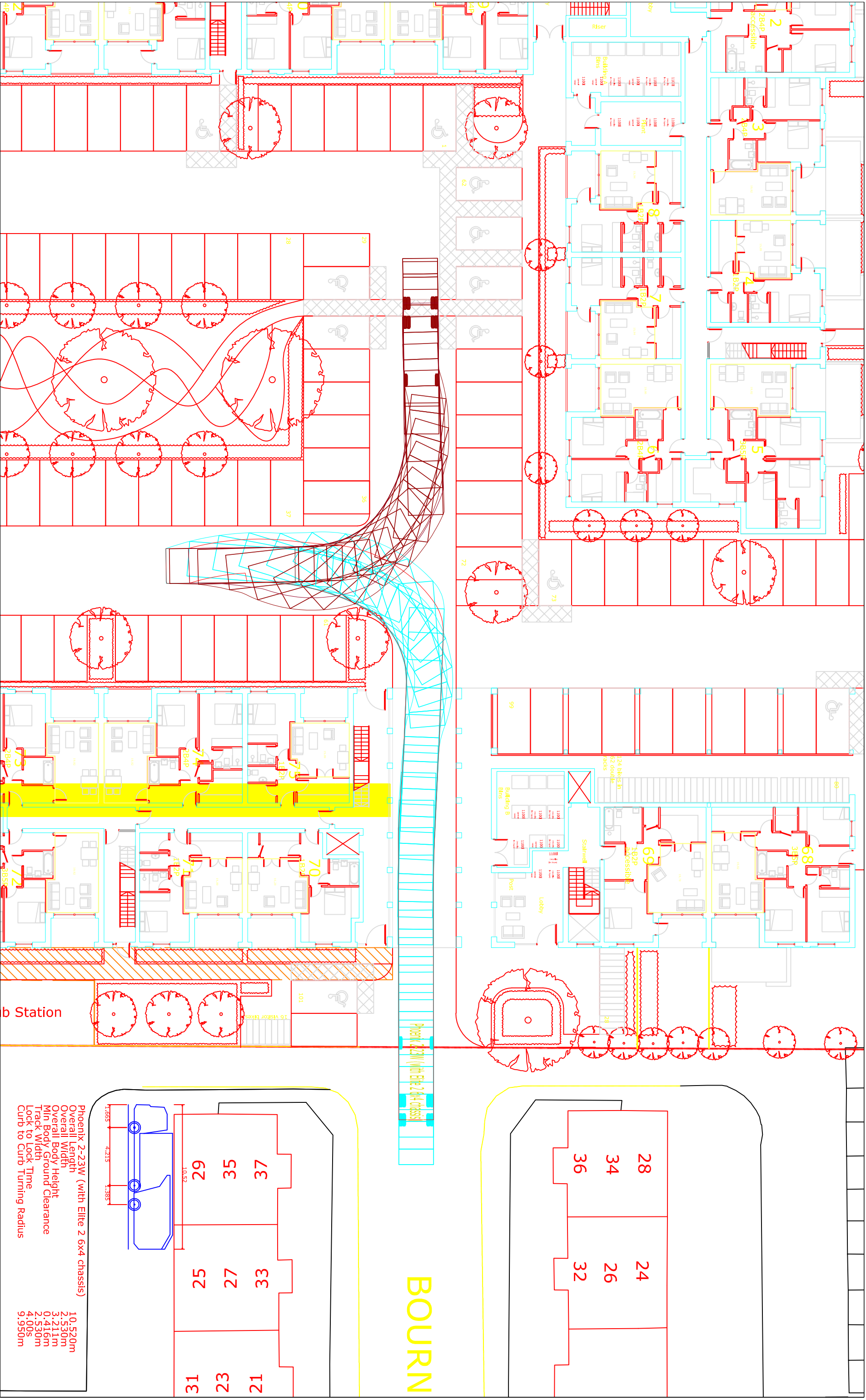
P1953: BOURNE COURT, RUISLIP Figure . AutoTrack; Hillingdon Council Refuse Vehicle Three-Point-Turn
