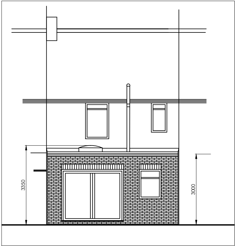
PROP REAR ELEV
