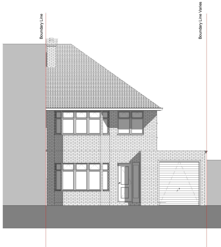
1 Front Elevation 1 Existing 1 : 100
