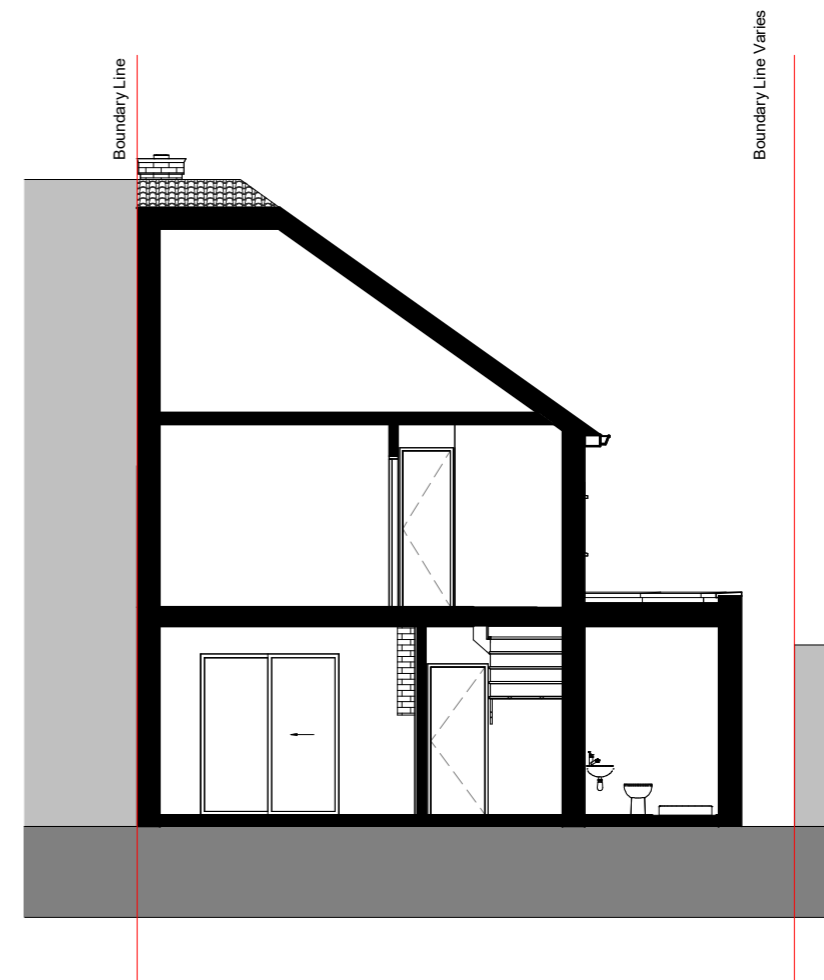
2 Proposed - Section 1 1 : 100
