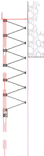
TYPICAL FACE FIXED INSTALLATION
