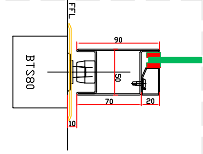
Head 1:4
