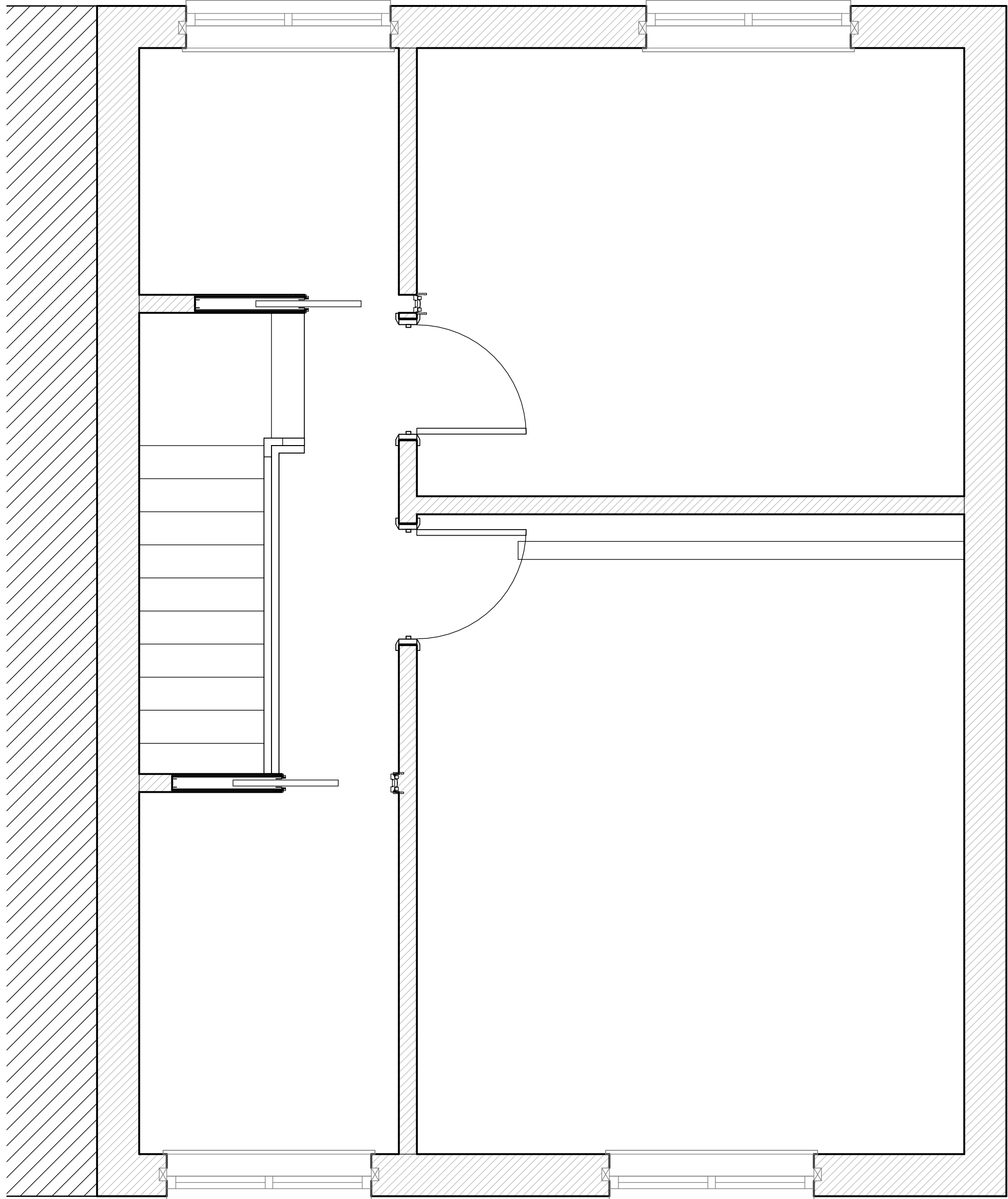
2 01_Existing First Floor Plan 1 : 25
