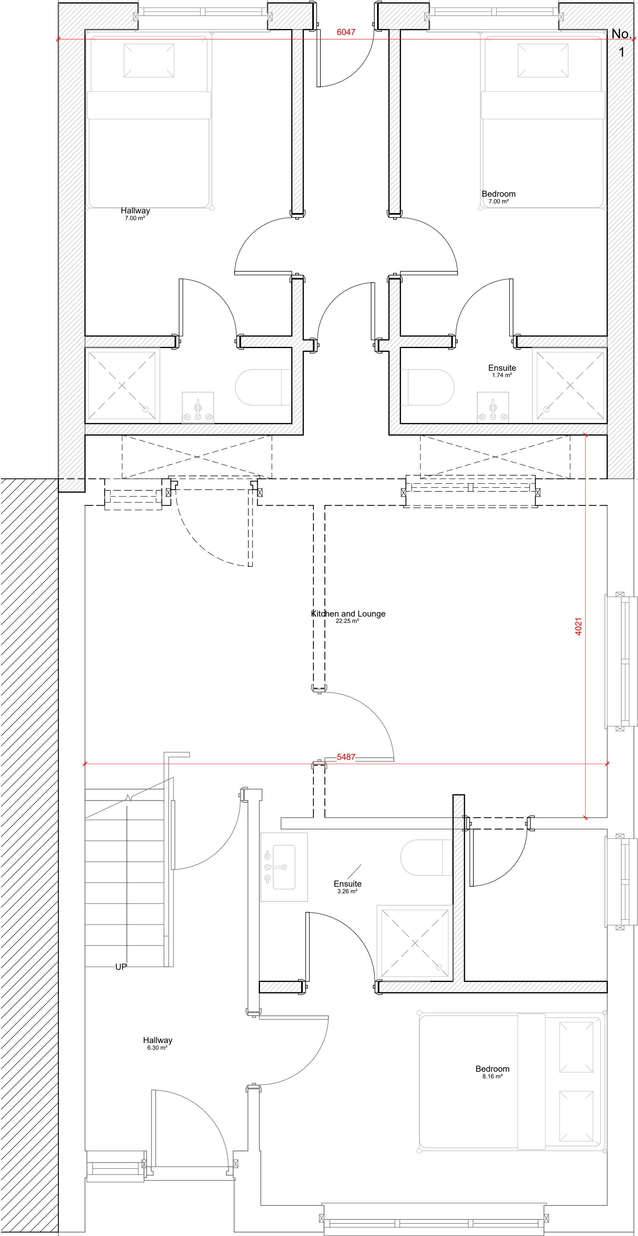
2 Proposed Ground Floor Plans 1 : 25
