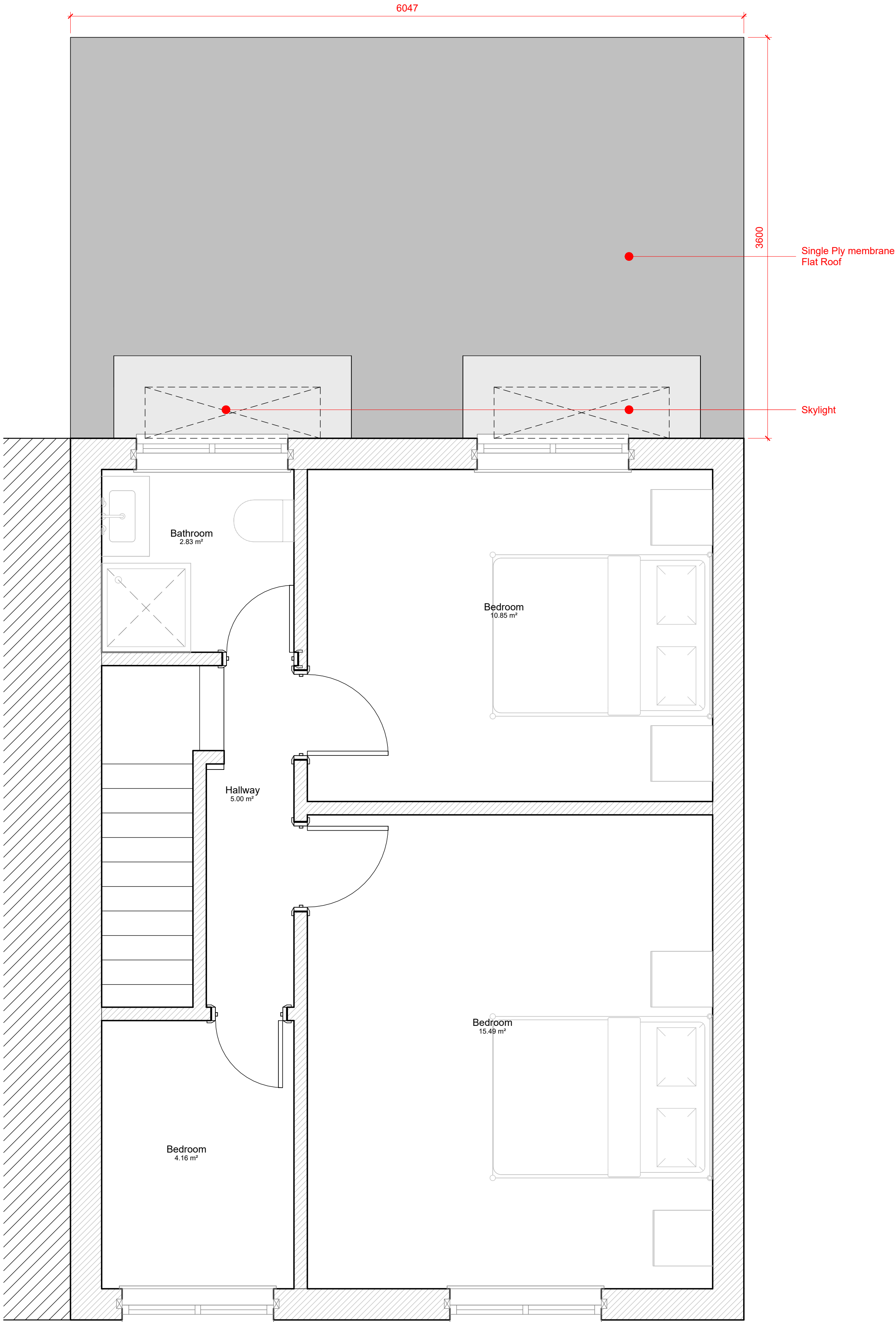
1 Proposed First Floor Plan 1 : 25
