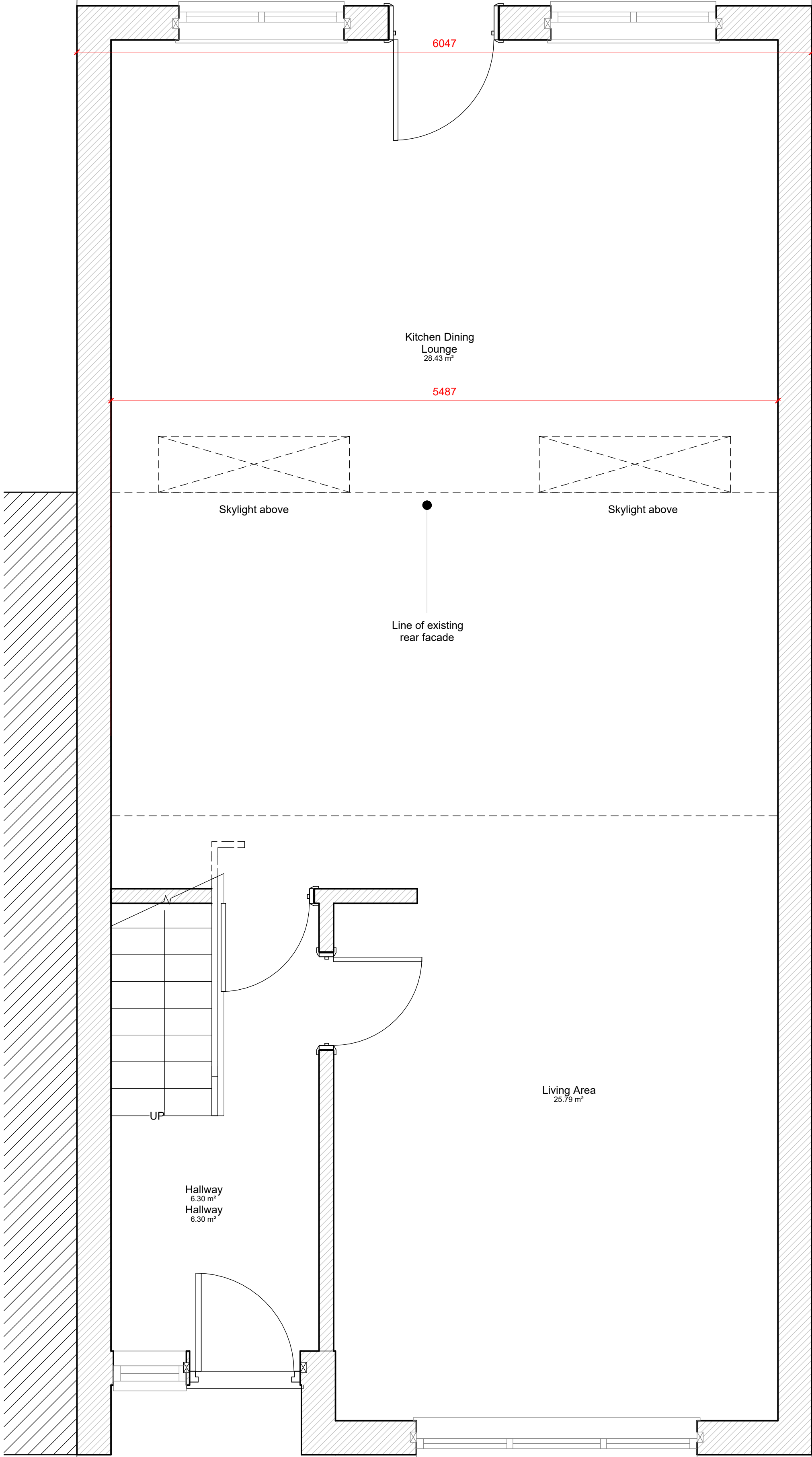
2 Proposed Ground Floor Plans 1 : 25
