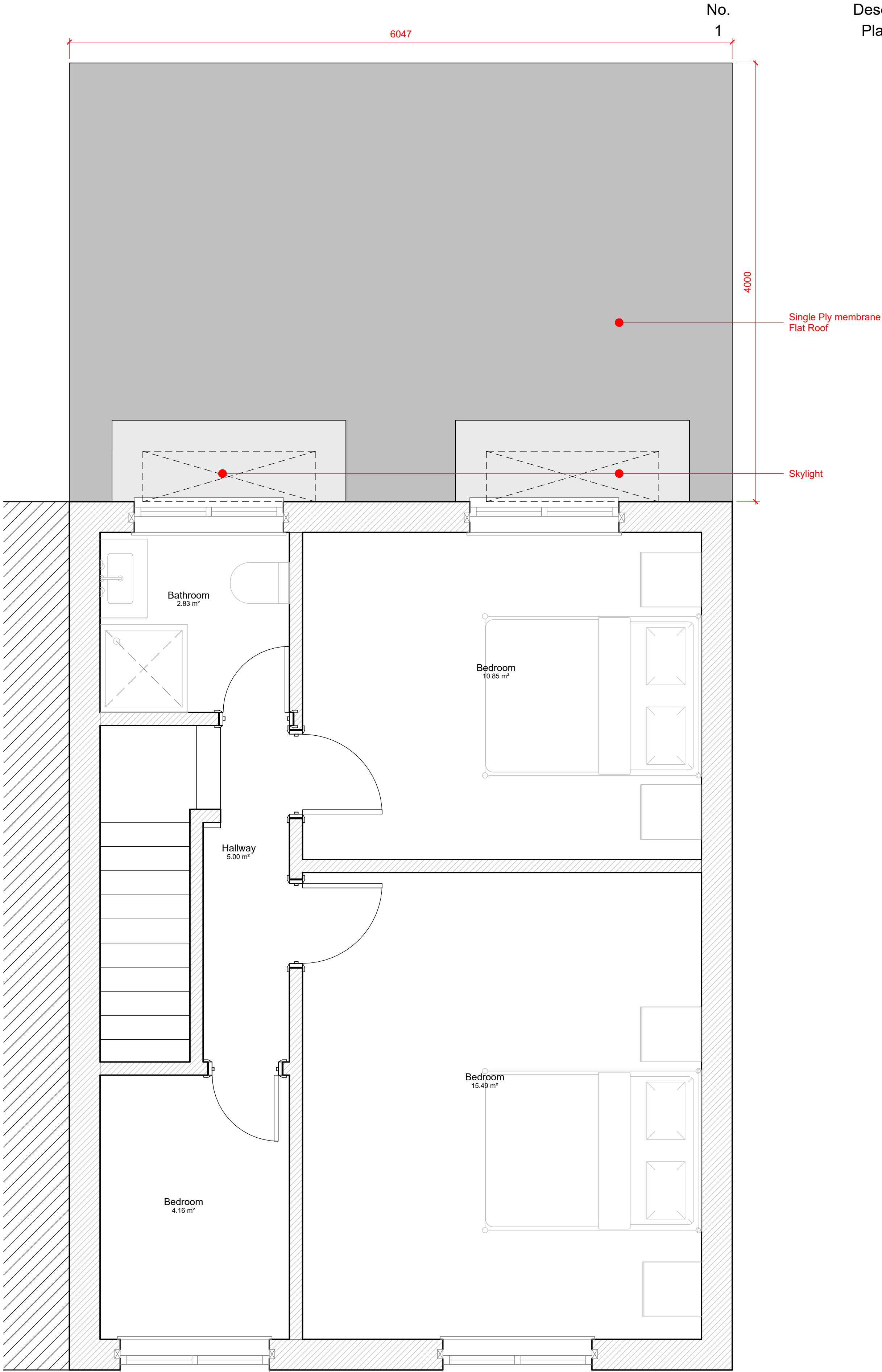
1 Proposed First Floor Plan 1 : 25
