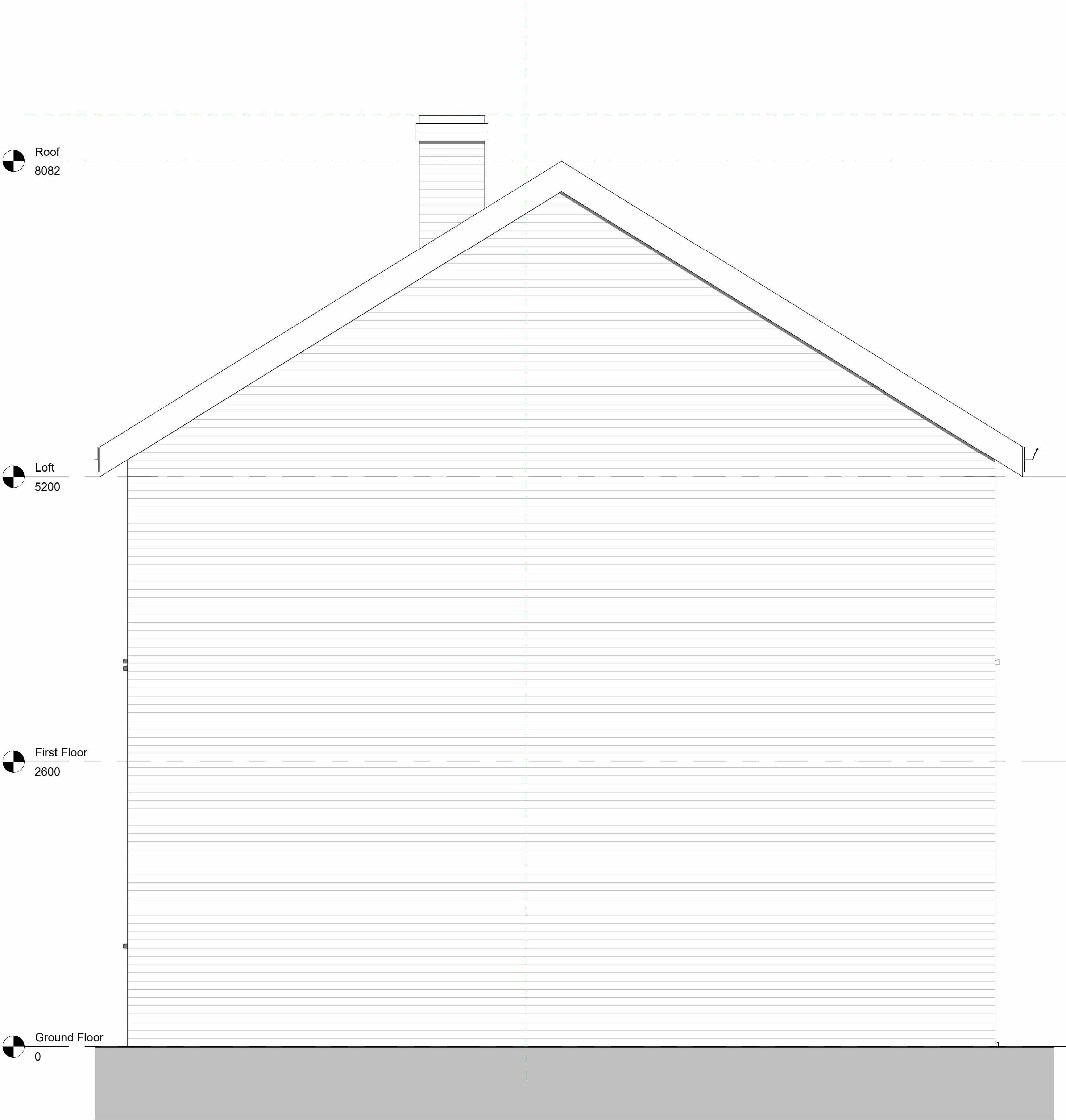
Existing Side Elevation 1 : 25
