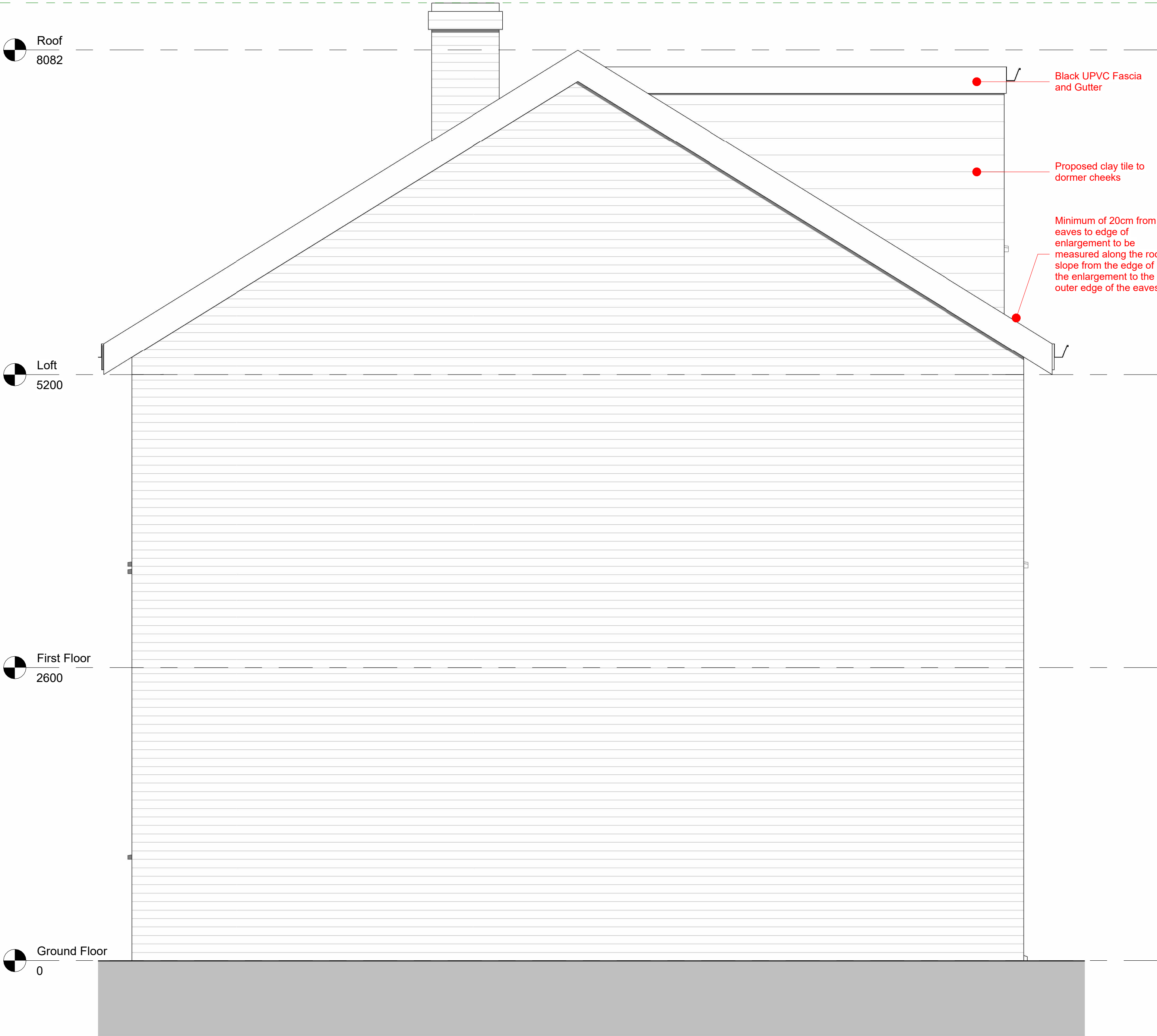
Proposed Side Elevation 1 : 25
