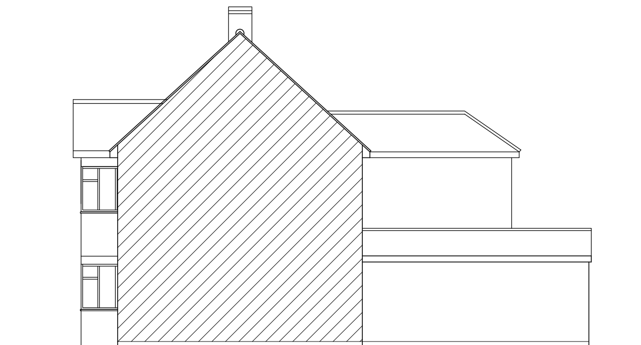
SIDE ELEVATION THROUGH PARTY WALL
