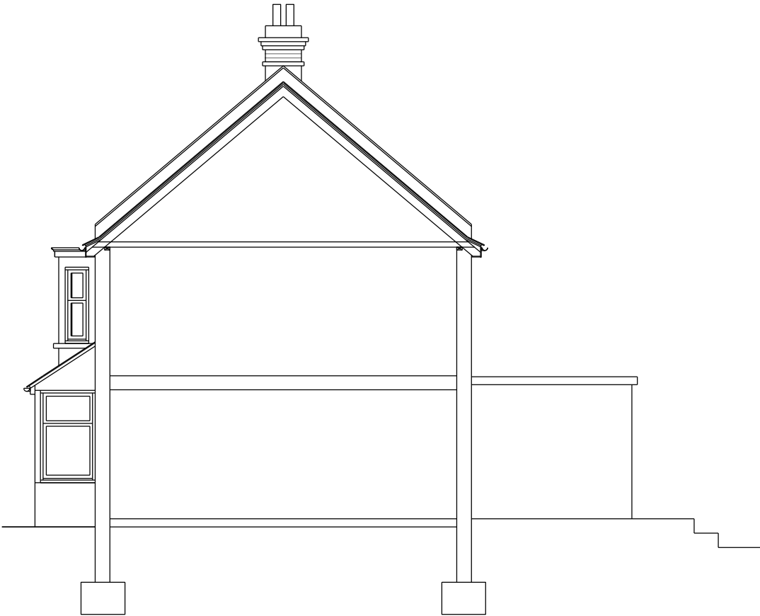
Pre-Existing Side Elevation/Section
