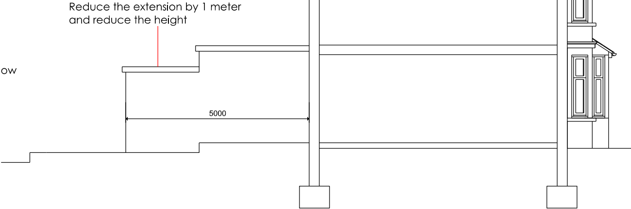
Proposed Side Elevation/Section
