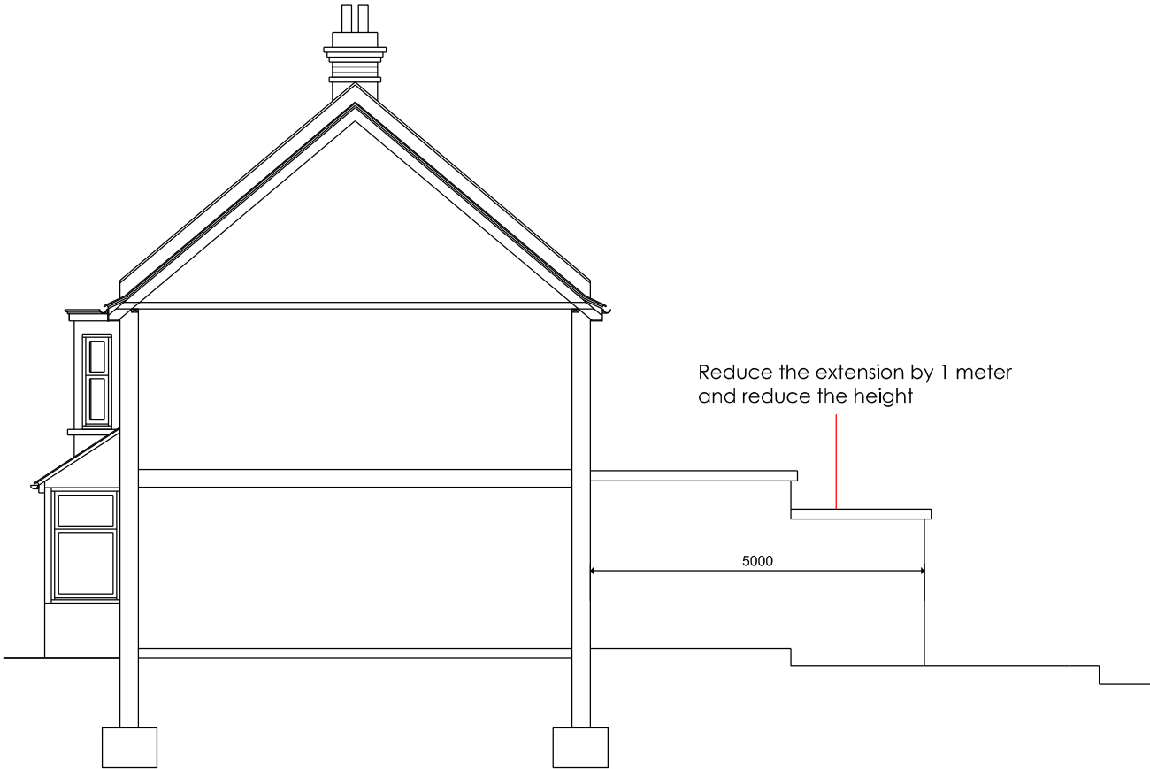
Proposed Side Elevation/Section
