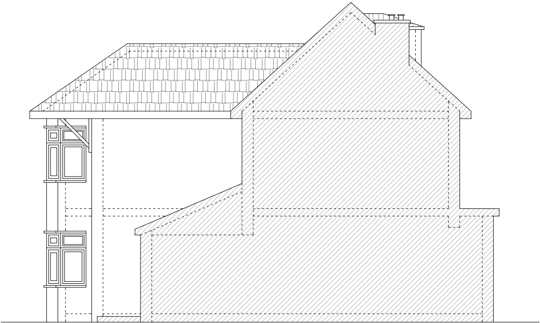
SOUTH EASTERN ELEVATION
