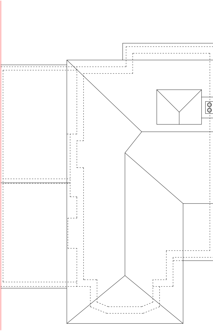
ROOF PLAN
