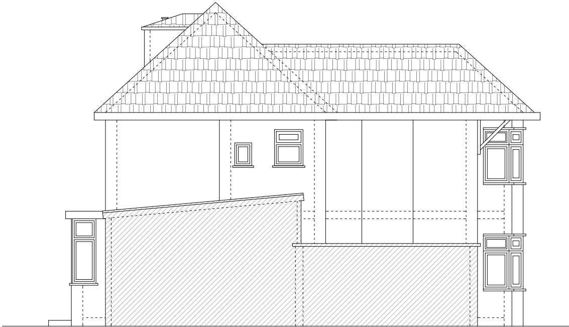
NORTH WESTERN ELEVATION
