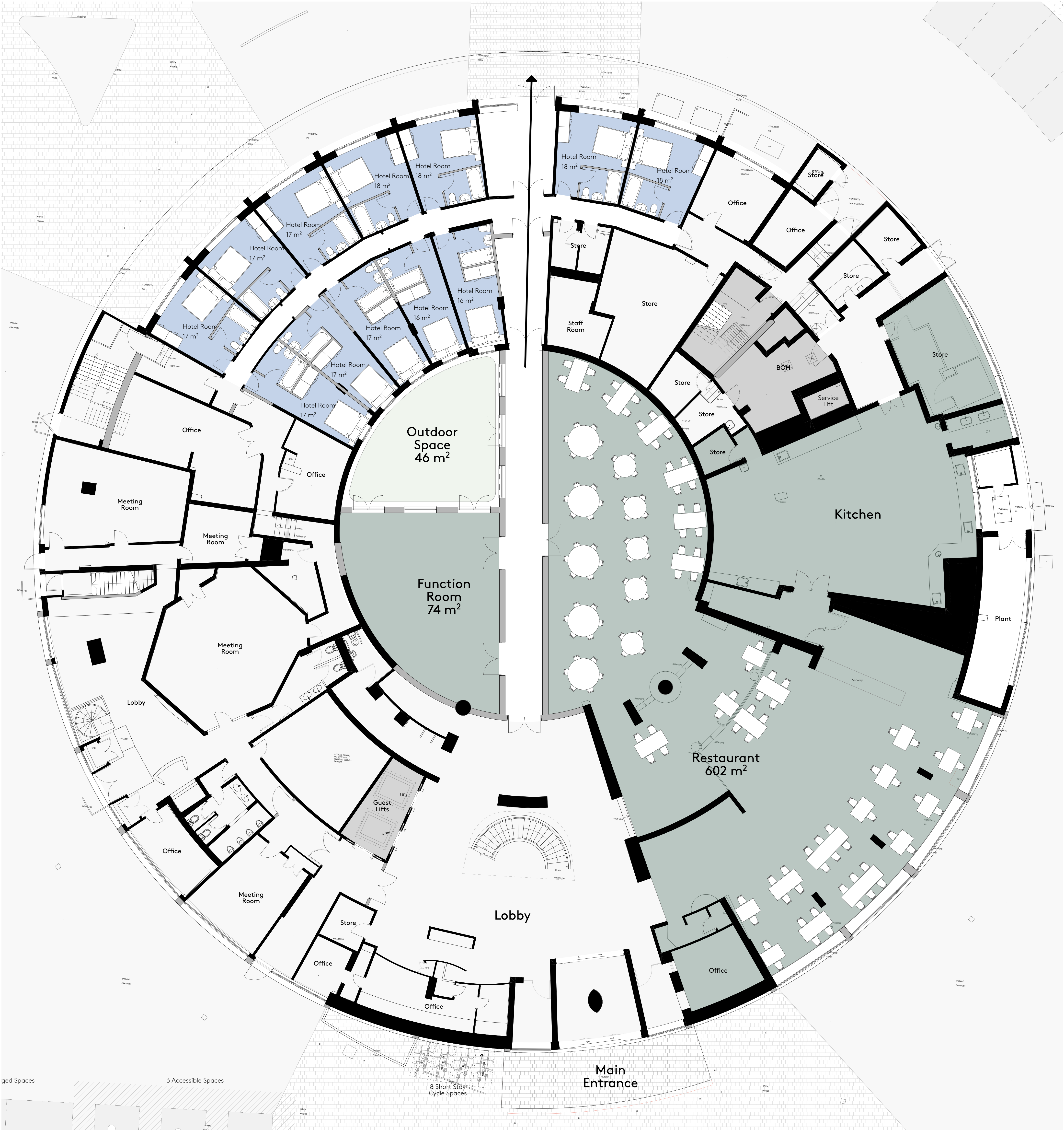
Proposed Ground Floor
