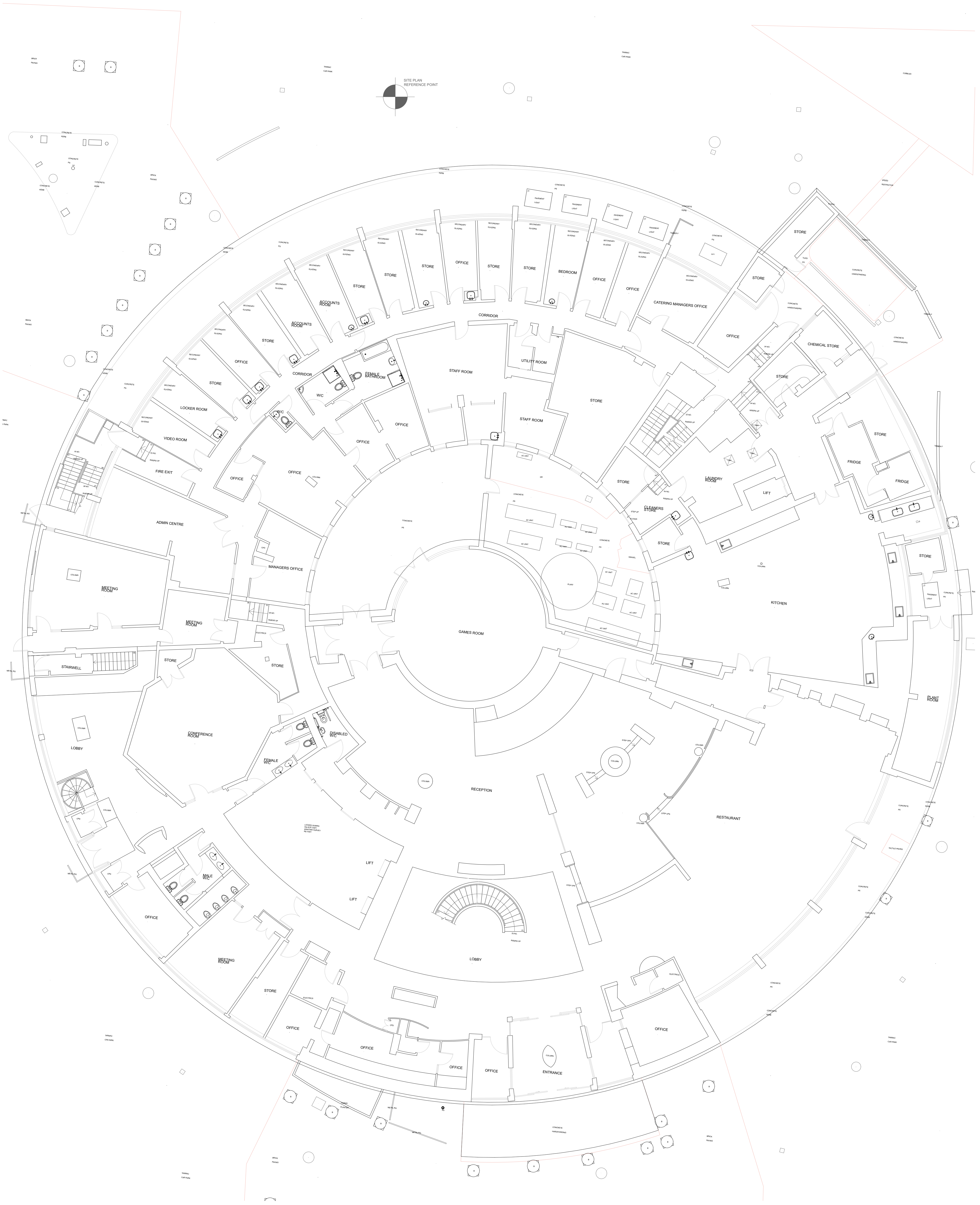
Existing Ground Plan
