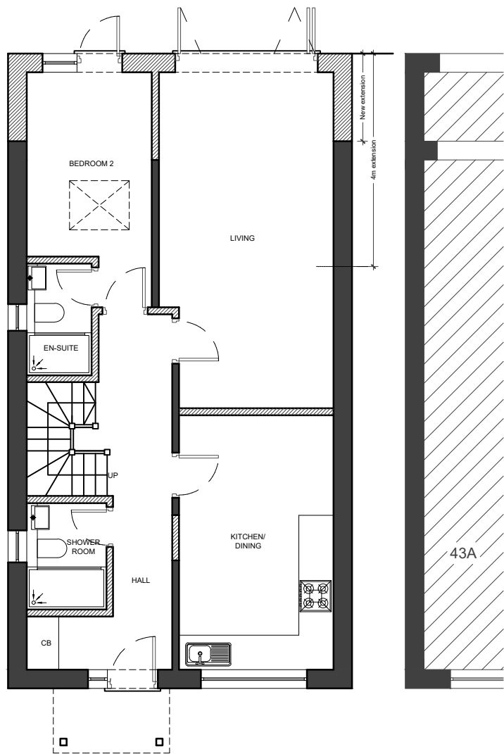
01 - GROUND FLOOR PLAN
