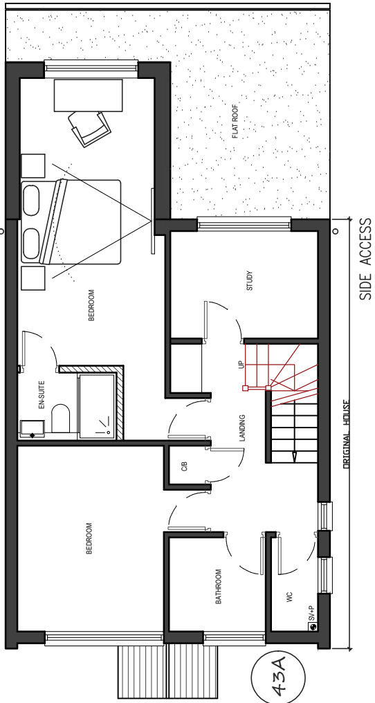
02-FIRST FLOOR PLAN
