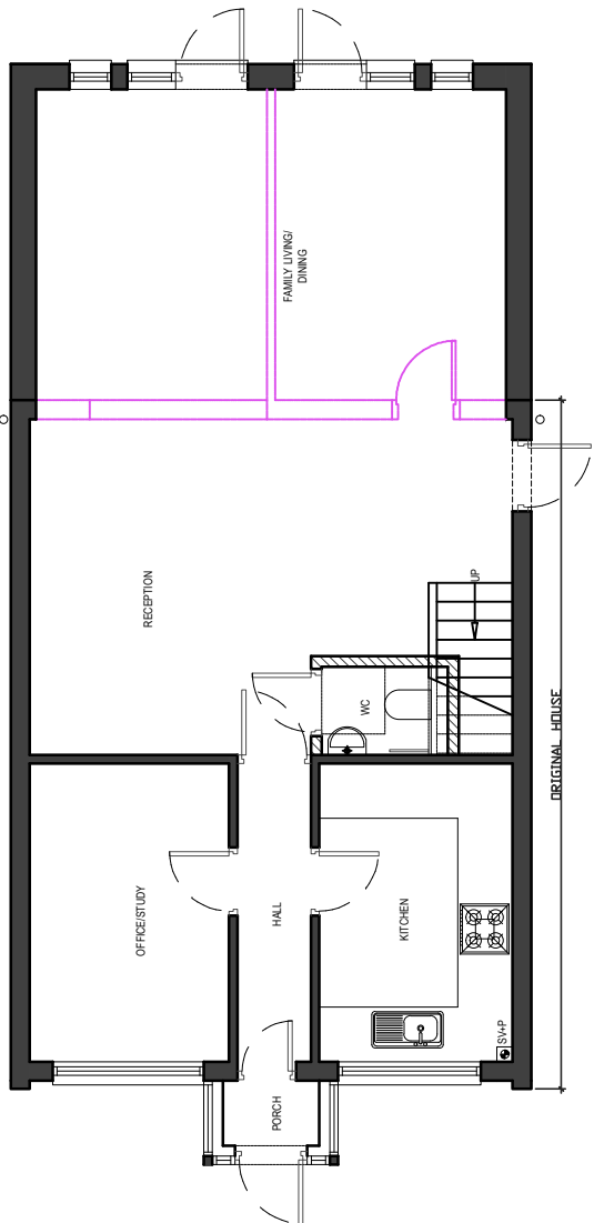
01- GROUND FLOOR PLAN
