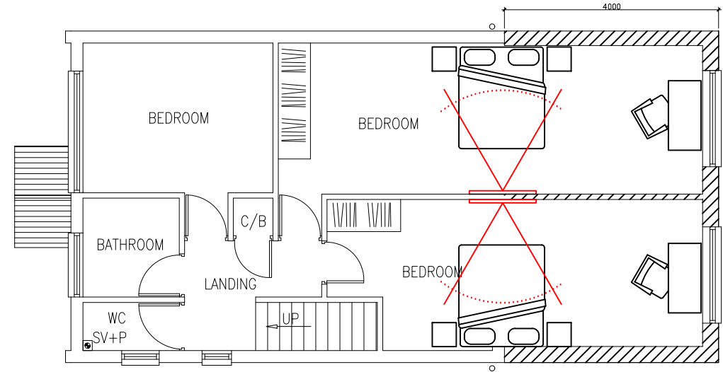
Proposed First Floor
