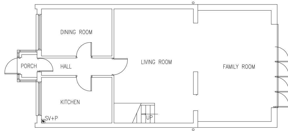
Proposed Ground Floor NO CHANGE
