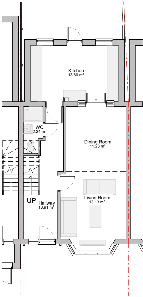
0 - Existing Ground Floor Plan 1 : 100
