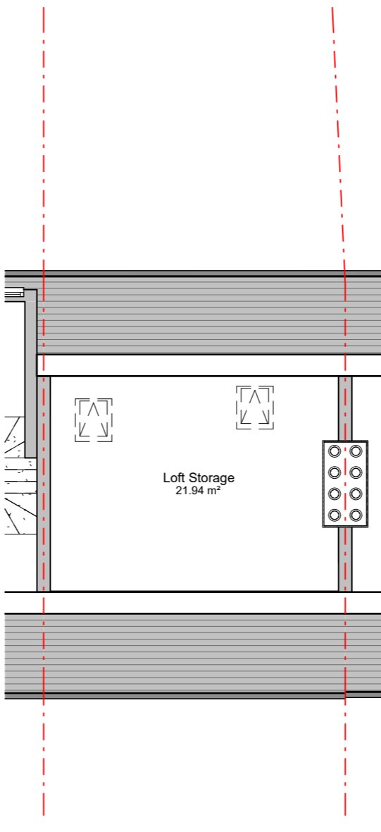
2 - Existing Second Floor Plan 1 : 100
