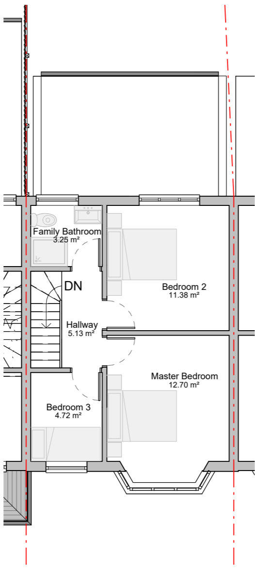
1 - Existing First Floor Plan 1 : 100
