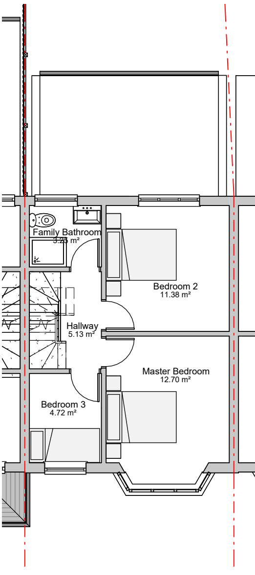
1 - Proposed First Floor Plan 1 1 : 100
