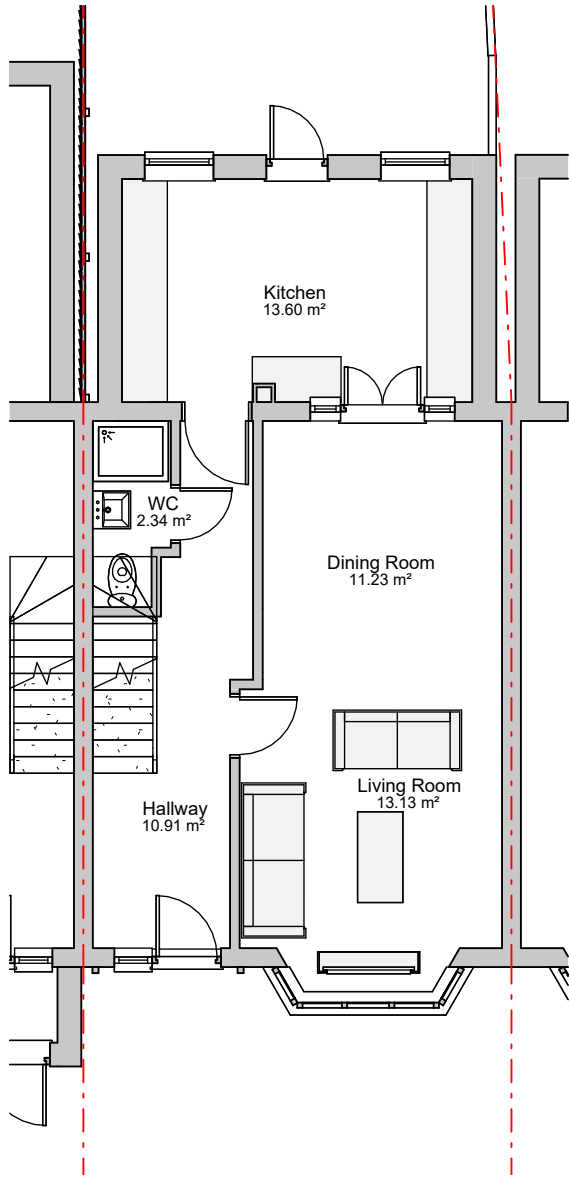
0 - Proposed Ground Floor Plan 1 1 : 100
