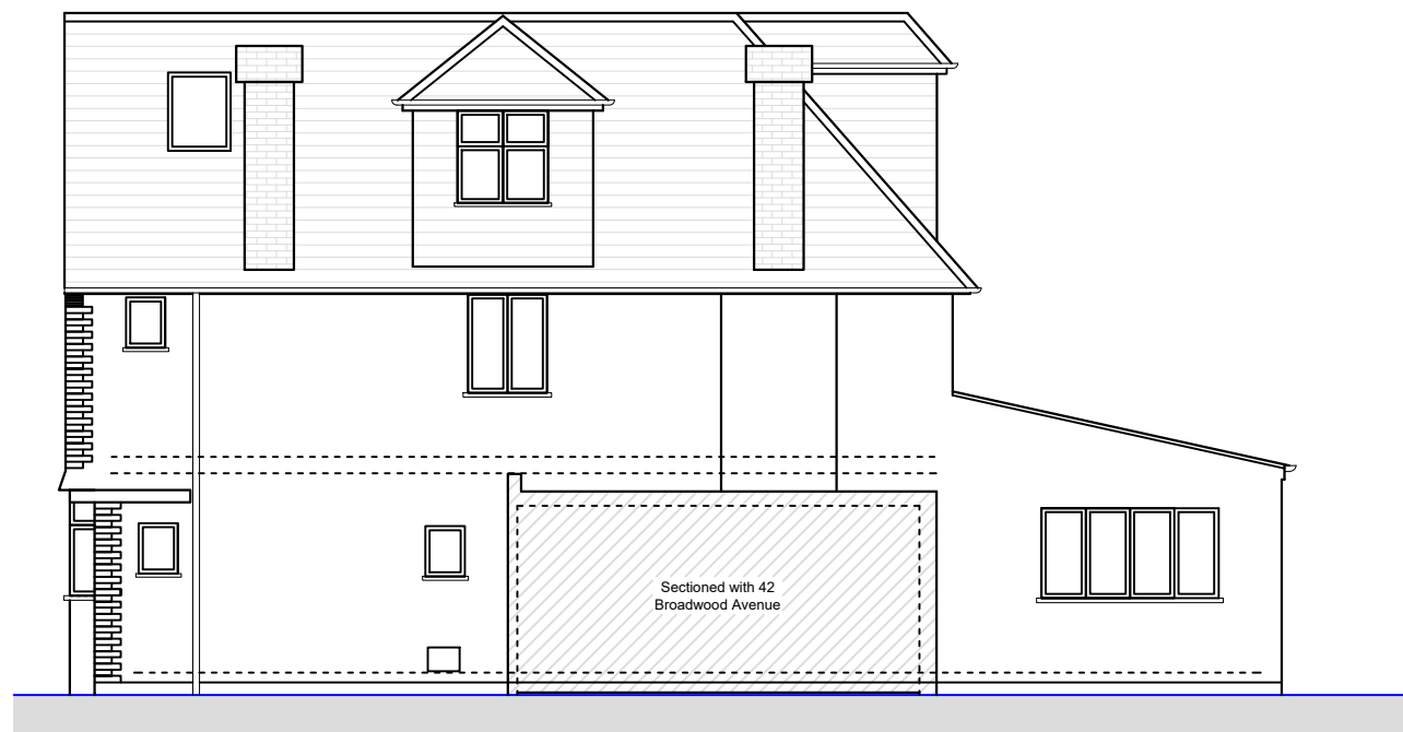
○ Side Elevation 1 1:100
