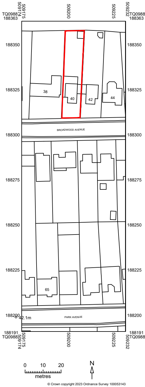
Location Plan 1 : 1 2 5 0
