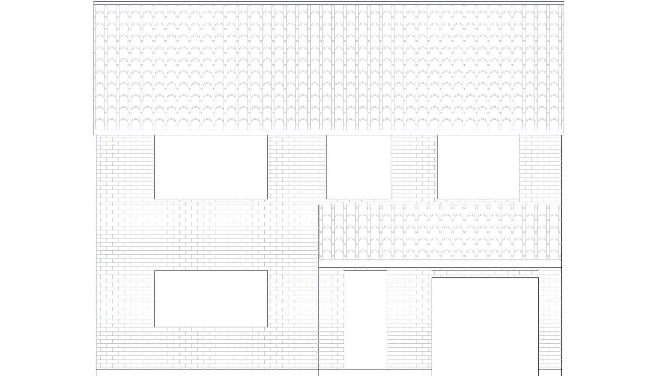
FRONT ELEVATION
