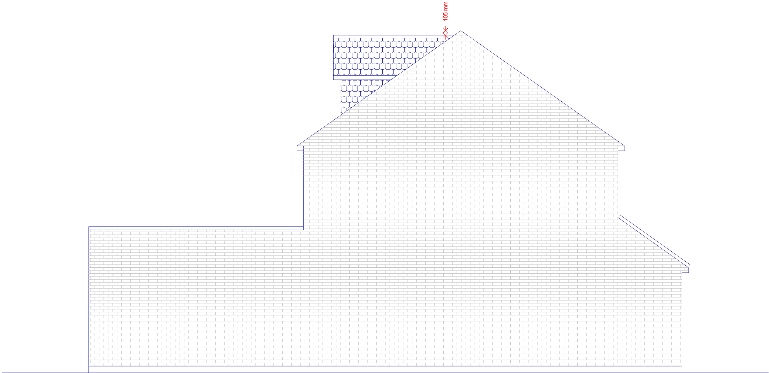
SIDE ELEVATION
