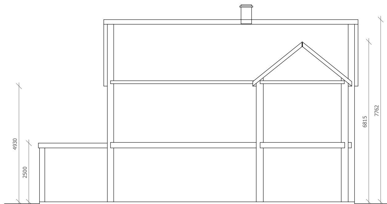
EXISTING SECTION
