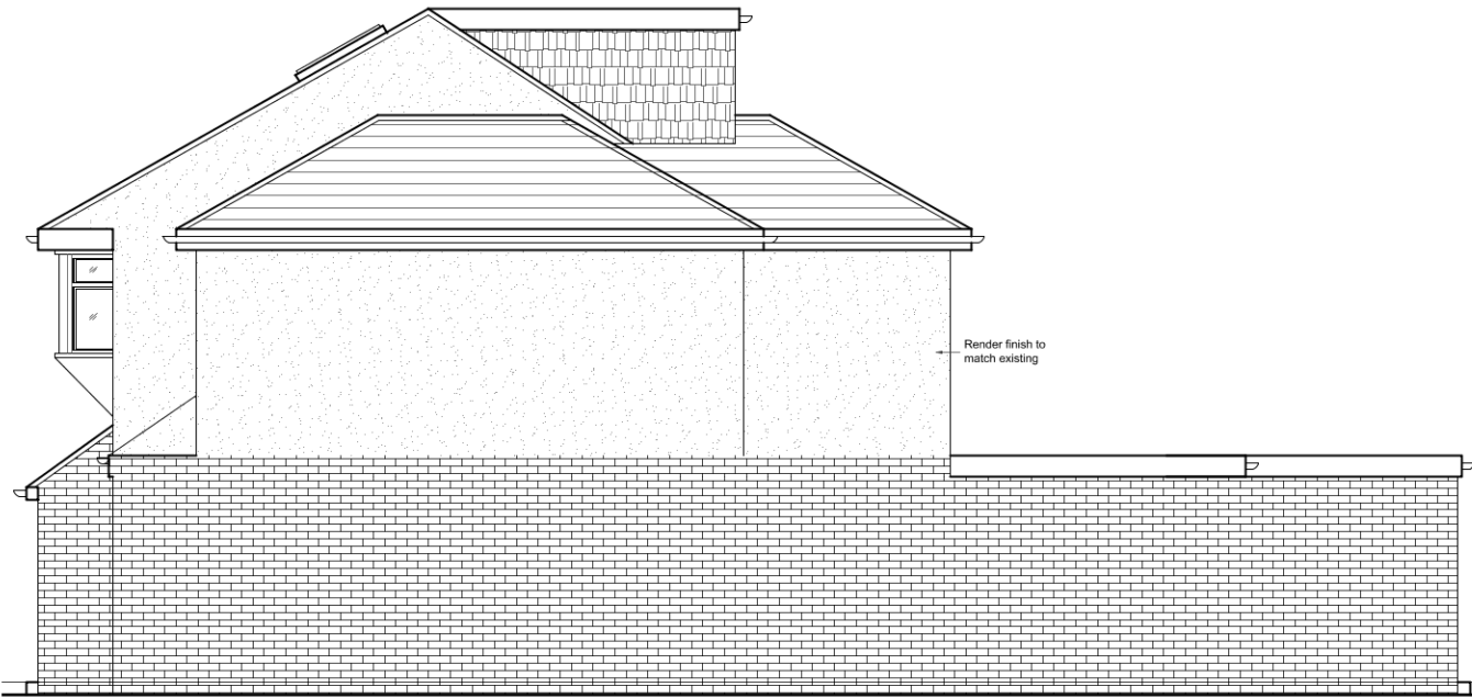
03 - SIDE ELEVATION
