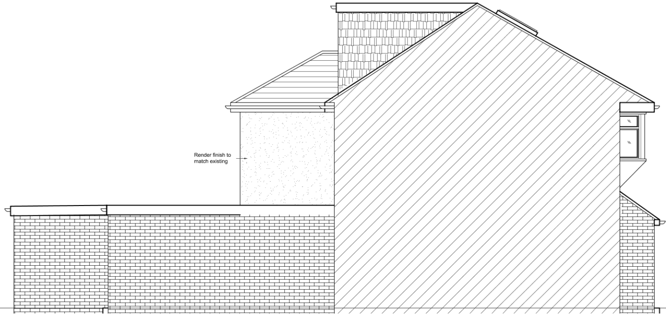
04 - OTHER SIDE ELEVATION
