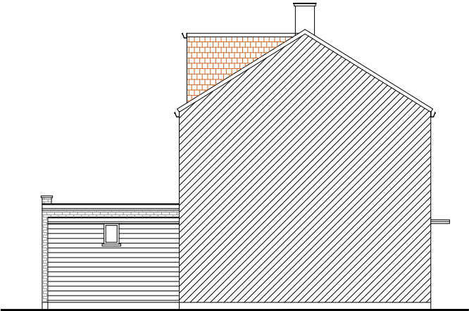
PROPOSED SIDE ELEVATION-2
