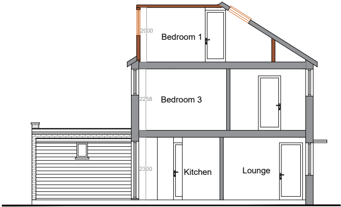
PROPOSED SECTION AA'
