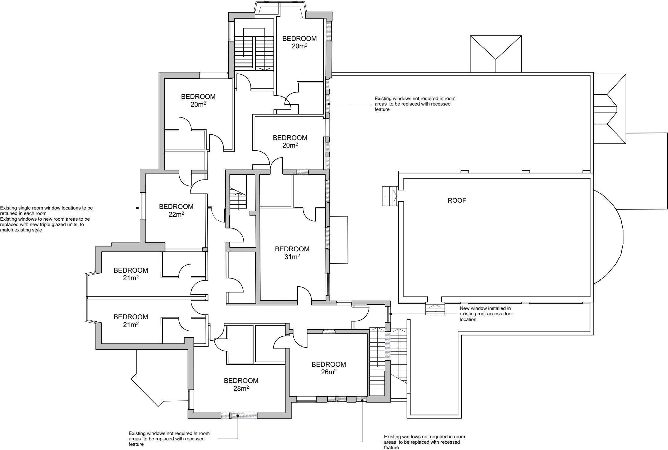
1 Proposed First Floor Plan Scale: 1:150
