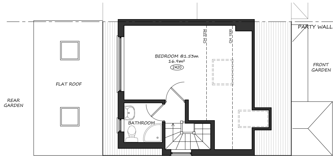
PROPOSED SECOND FLOOR PLAN 1:100
