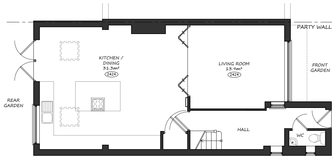
PROPOSED GROUND FLOOR PLAN 1:100
