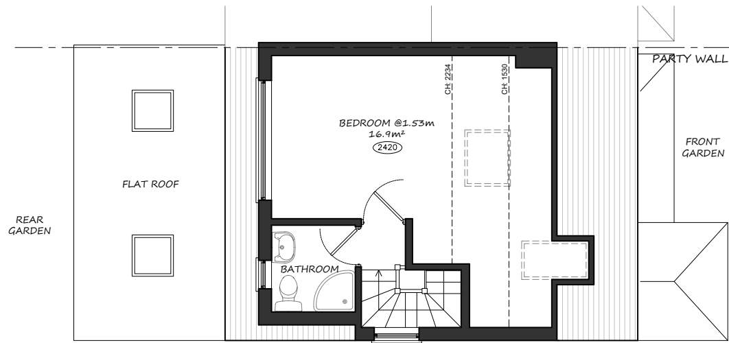
EXISTING SECOND FLOOR PLAN 1:100
