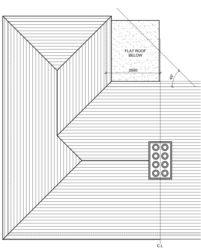
03 - ROOF PLAN
