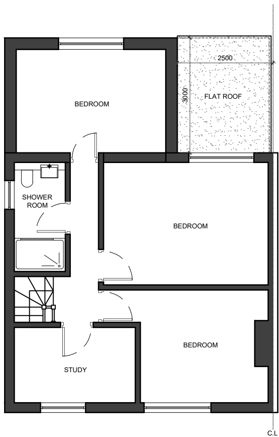
02 - FIRST FLOOR PLAN
