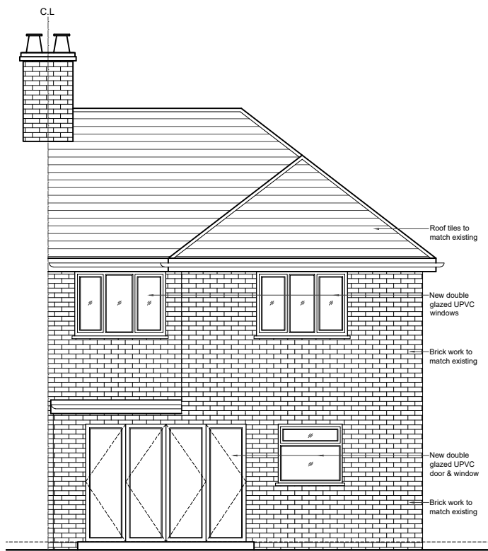
05 - REAR ELEVATION
