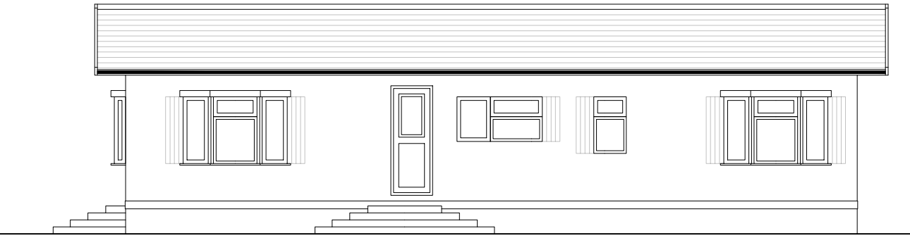
EXISTING SIDE ELEVATION 1:100
