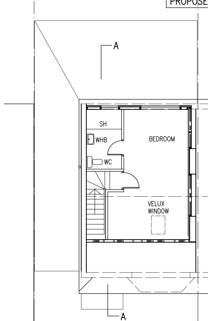
LOFT FLOOR PLAN
