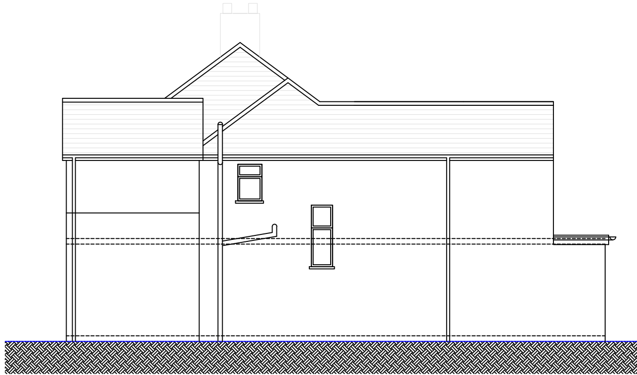
○ Side Elevation 1 : 1 0 0
