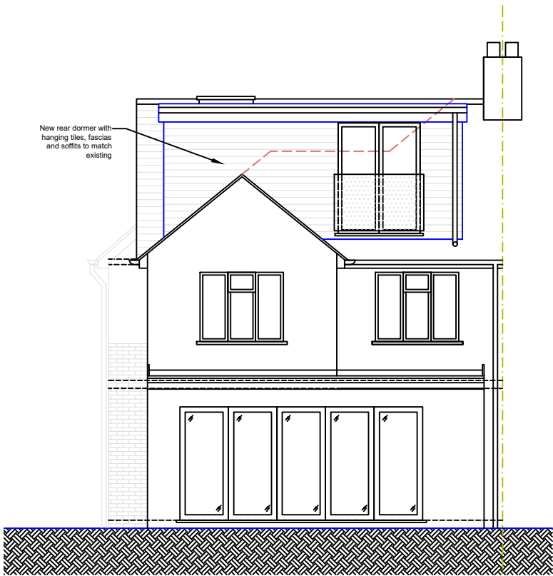
○ Rear Elevation 1 : 1 0 0
