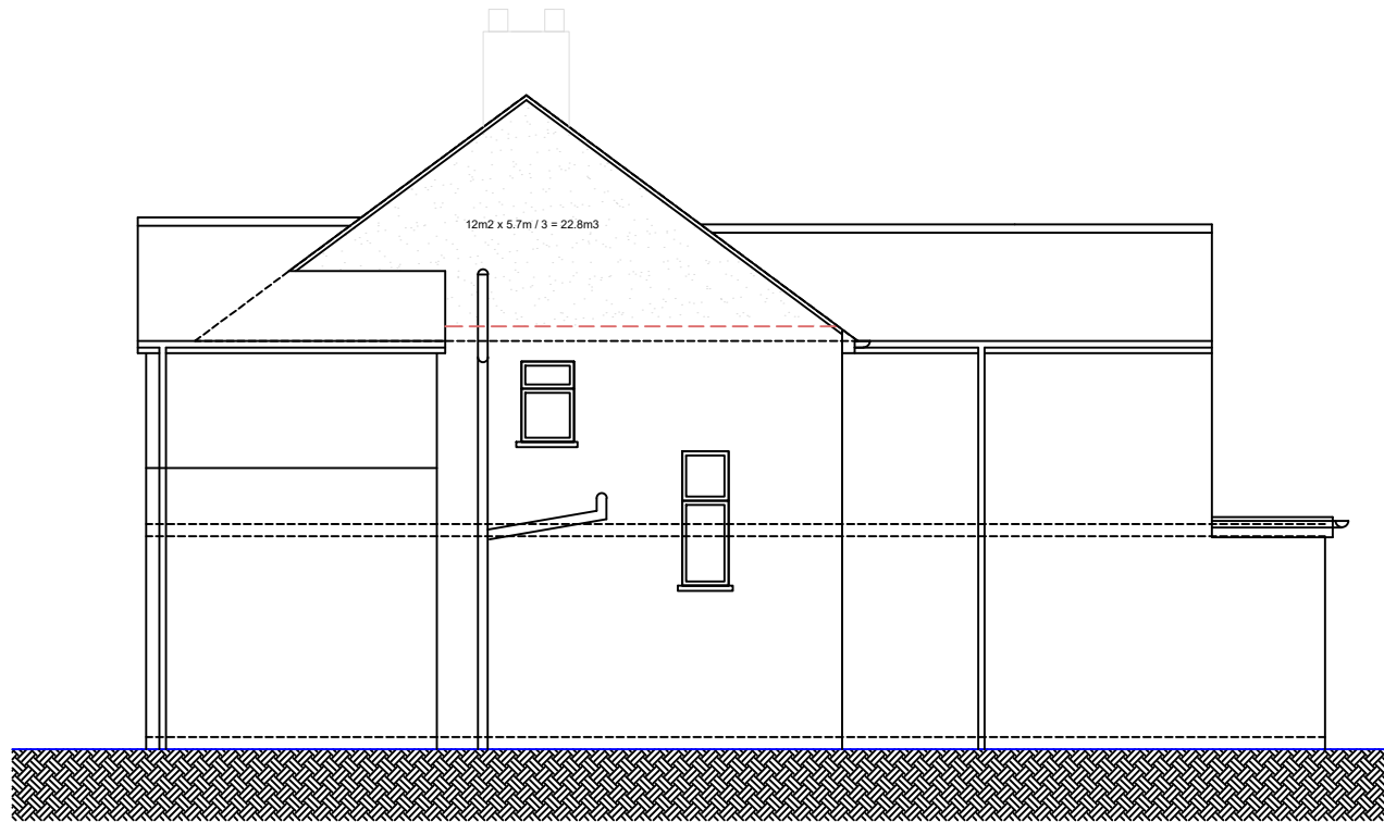
○ Side Elevation 1 : 1 0 0
