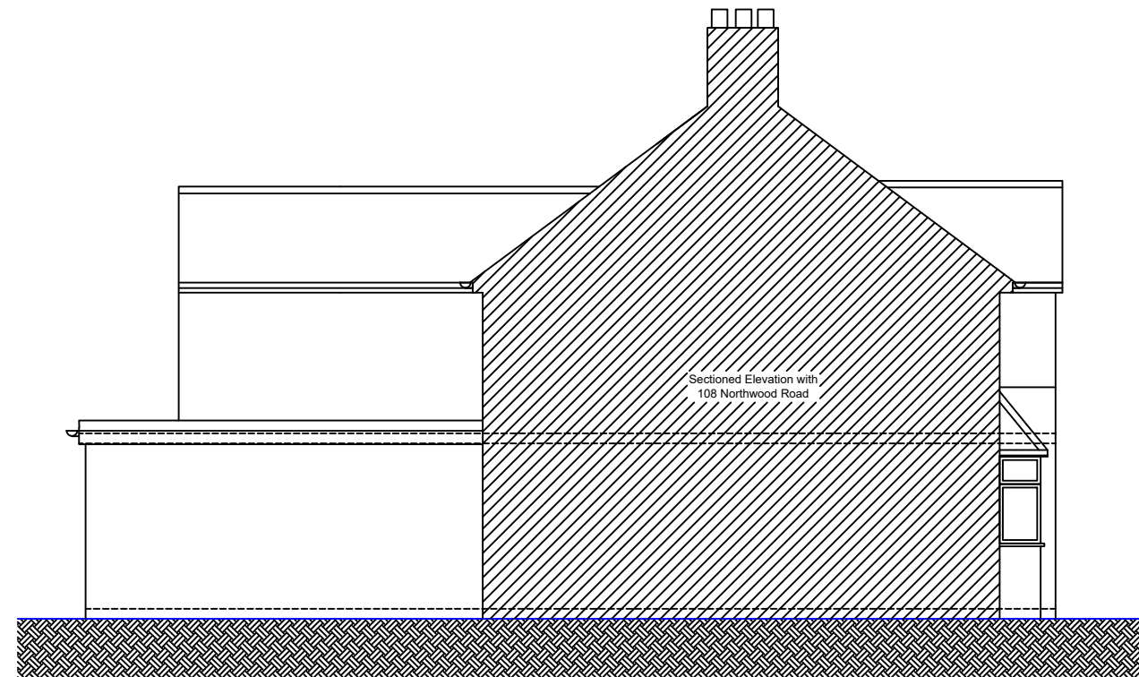
○ Sectioned Side Elevation 1 : 1 0 0
