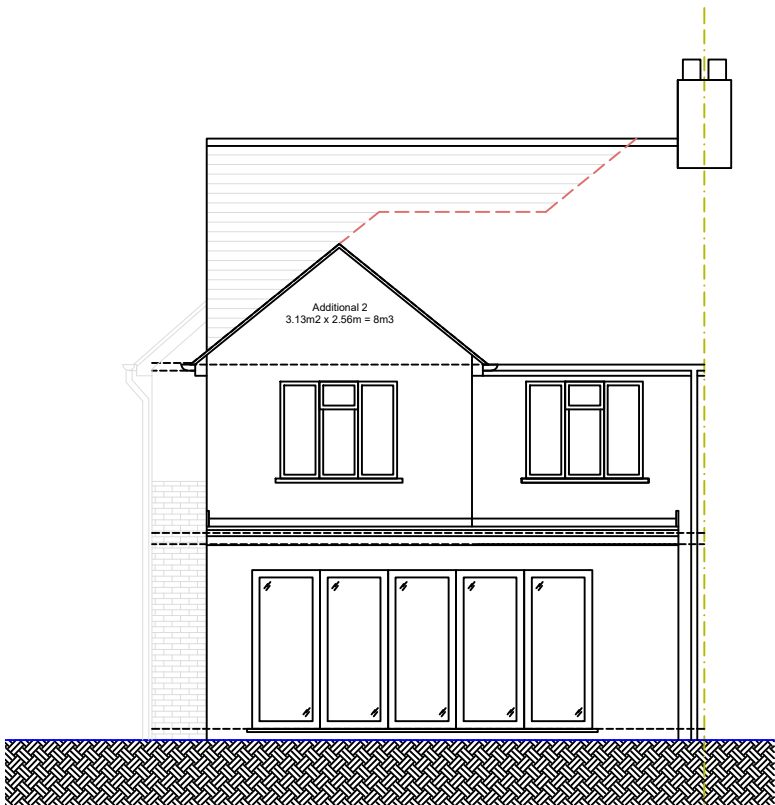
○ Rear Elevation 1 : 1 0 0
