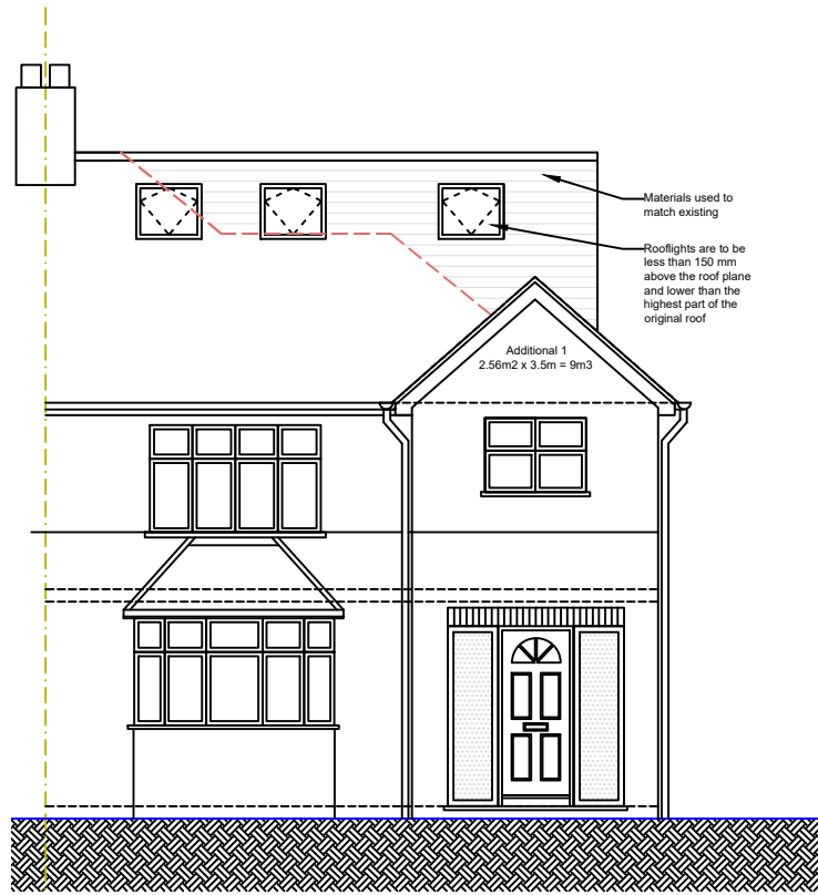
○ Front Elevation 1:100
