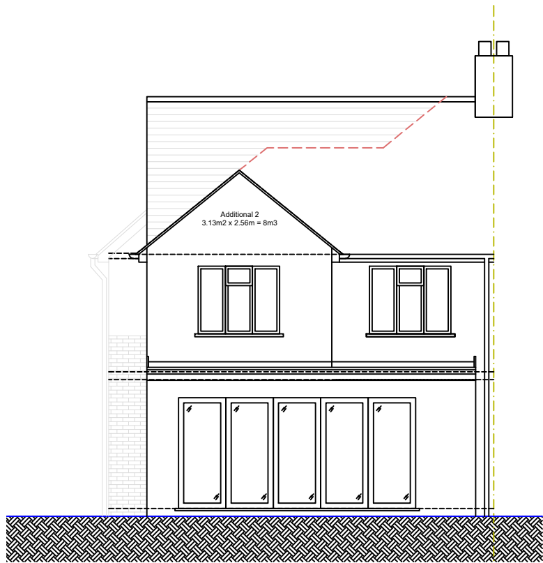
○ Rear Elevation 1:100
