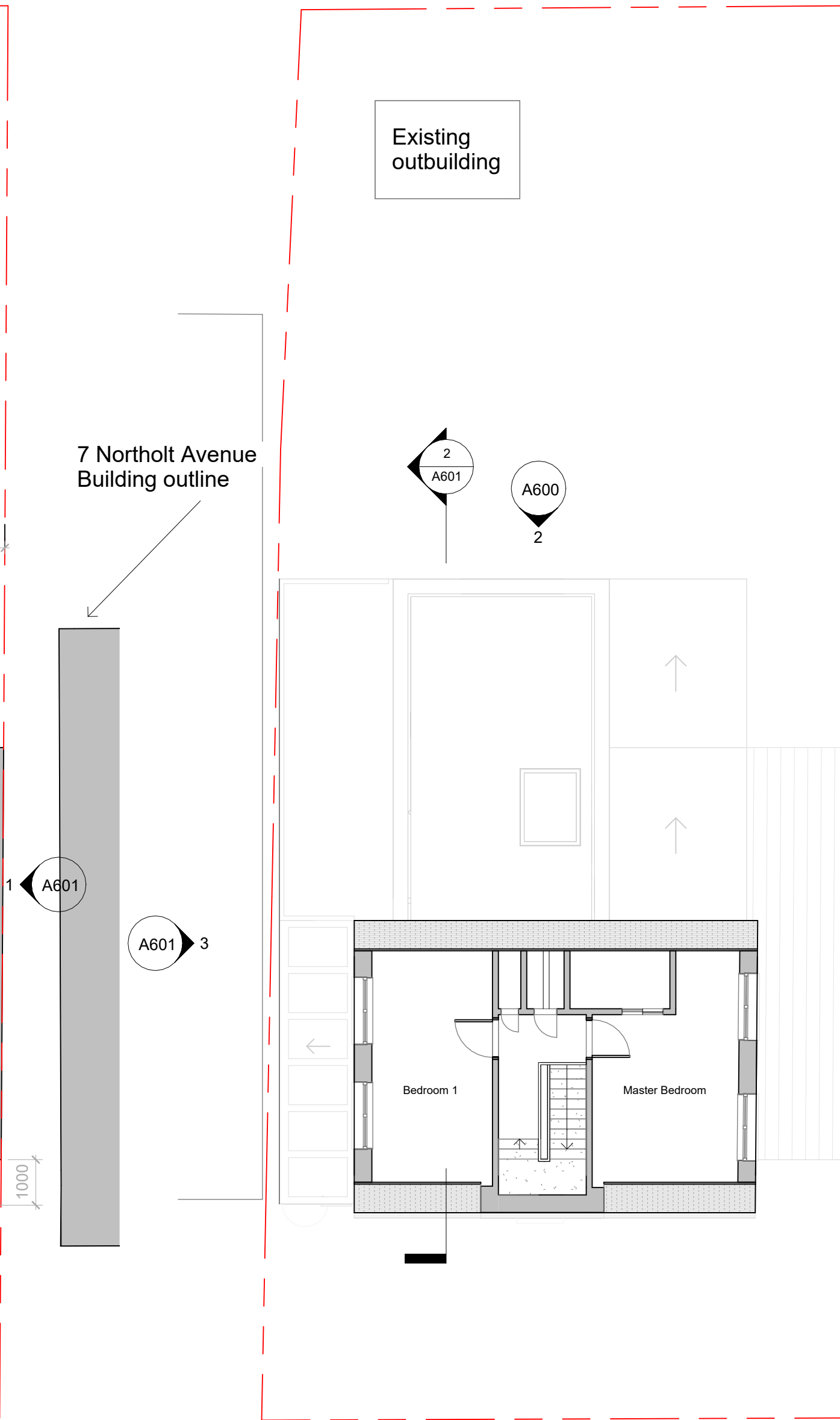
2 Proposed First Floor Plan (No Change) 1 : 100
