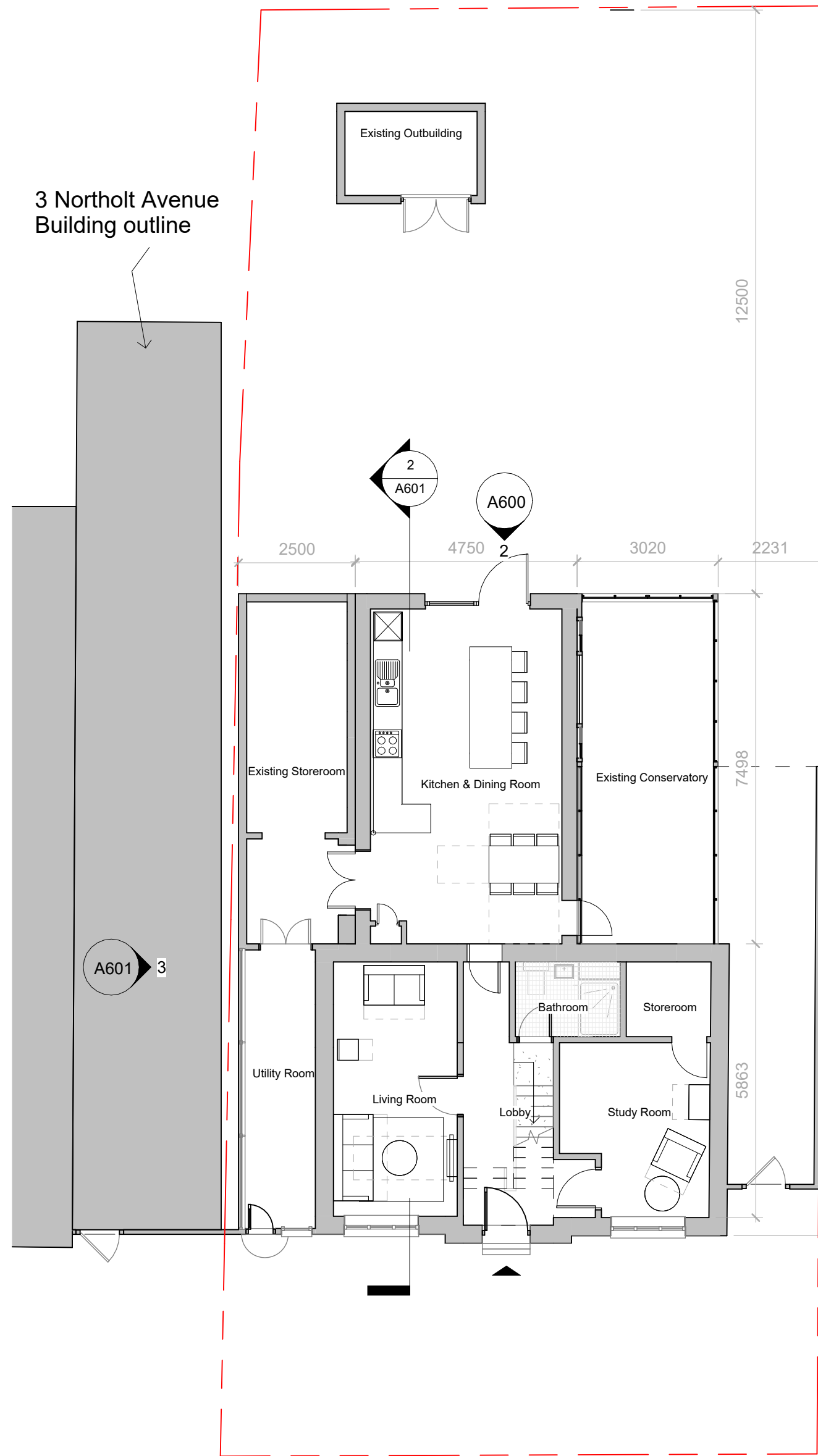
1 Proposed Ground Floor Plan 1 : 100
