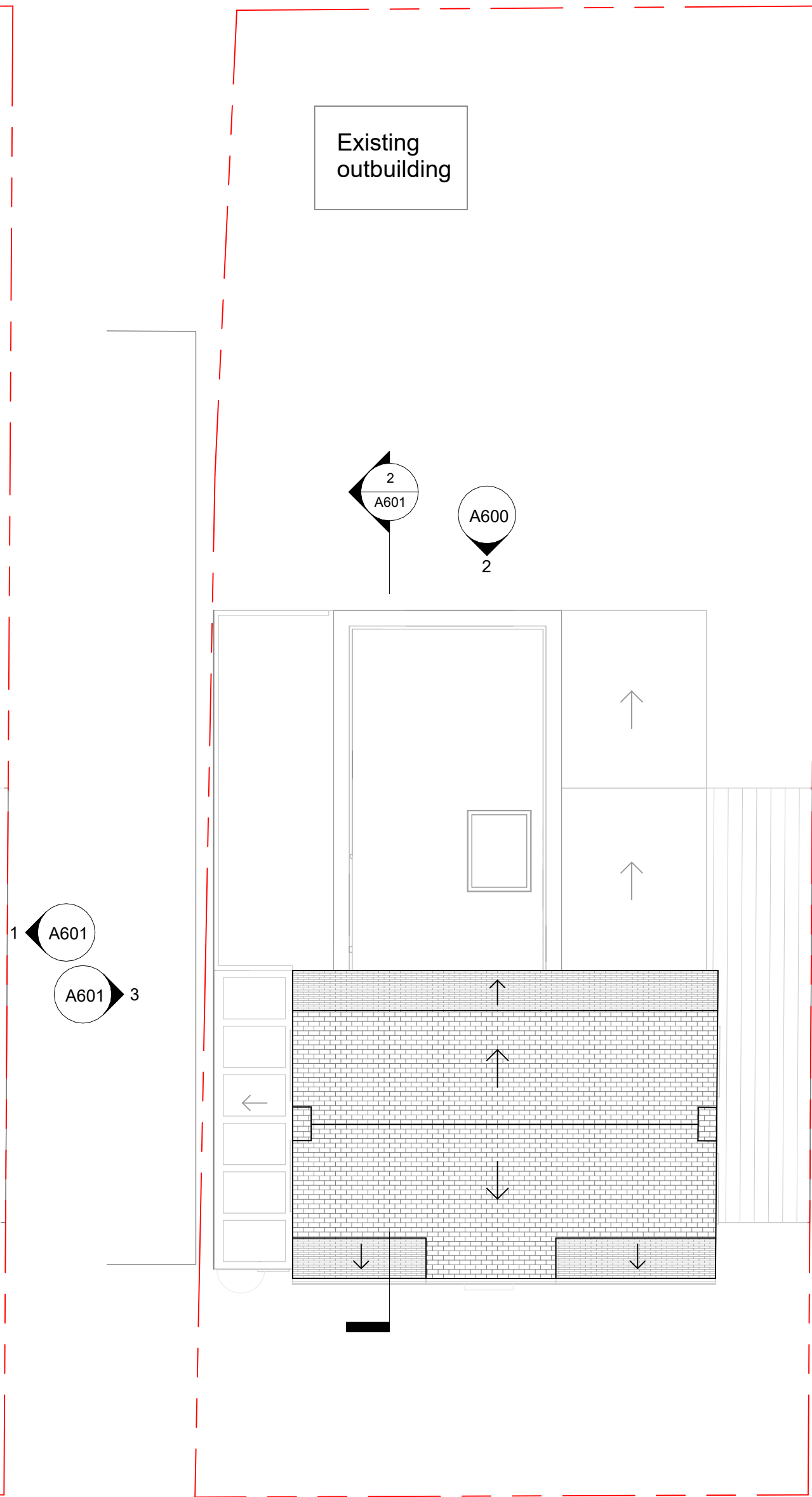
3 Proposed Roof Plan (No Change) 1 : 100
